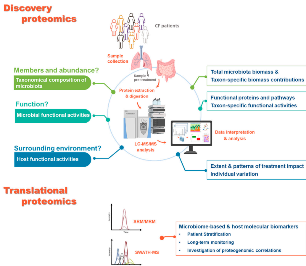
Figure 3. Questions that could be answered using proteomics-based approaches. Sample questions that could currently be addressed by analysing airways and intestinal microbiota from CF patients using proteomics-based approaches. For the discovery proteomics, for each question described (left side), the corresponding output of the metaproteomic analysis is summarised (right side). The main steps in the experimental workflow and the widely used approaches are also highlighted. For the translational proteomics, the main approaches are indicated alongside with their output.
