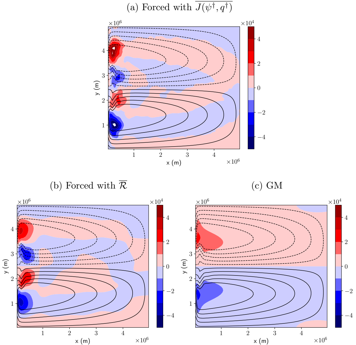
FIG. 14: Color: The difference in stream function between the coarse reference run with \overline{\mathcal{R}} = 0 and coarse runs with eddy closures ( [m^2 s^{-1}] ). Contours: Stream function of the low resolution REF run. The run with \overline{J(\psi^\dagger, q^\dagger)} smoothed by 16 neighboring grid points (a), with \overline{\mathcal{R}} (b), and with GM only (c).
