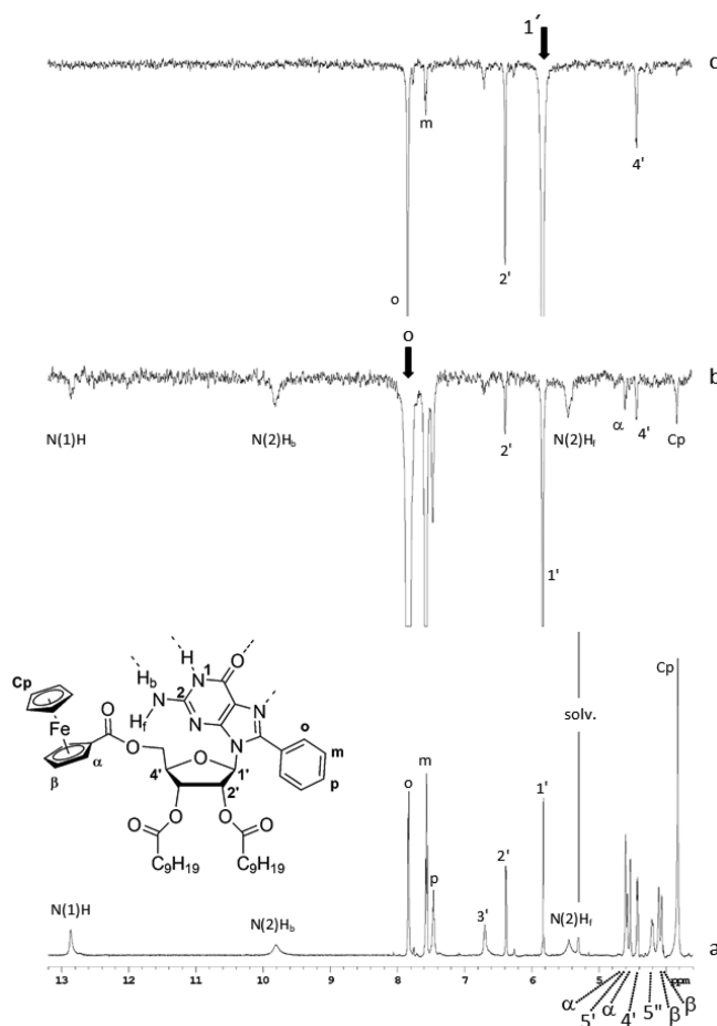
Figure 1. (a) Downfield portion of the 600 MHz ^1\text{H-NMR} spectrum of 8Ph5Fc in \text{CD}_2\text{Cl}_2 (4.3 mM) at -20 °C and signal assignment (diastereotopic protons were not assigned); (b) NOESY-1D spectrum of the same sample upon irradiation at 7.83 ppm (“o” protons); (c) NOESY-1D spectrum of the same sample upon irradiation at 5.82 ppm ( 1' proton). In each NOE spectrum were used 512 coadded transients, a recycle delay of 0.6 s, a mixing time of 0.6 s, and a 50 Hz shaped pulse. Irradiated frequencies are indicated with an arrow.
