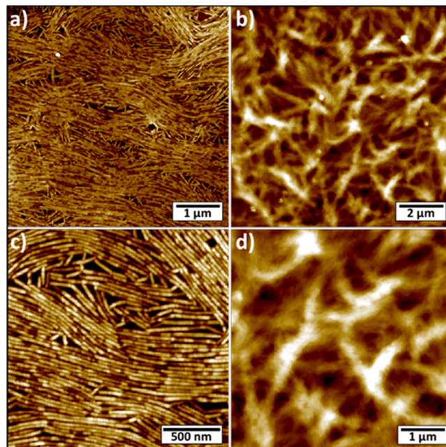
Figure 3. AFM images of supramolecular metal-free G aggregates drop-cast from CH_2Cl_2 0.6 mg/mL on HMDS-functionalized SiO_2 . (a,c) Molecule 8Ph5Fc . (b,d) Molecule 8Fc5C10 . Images Z-scales: (a) 10 nm; (b) 140 nm; (c) 7 nm; and (d) 110 nm.
