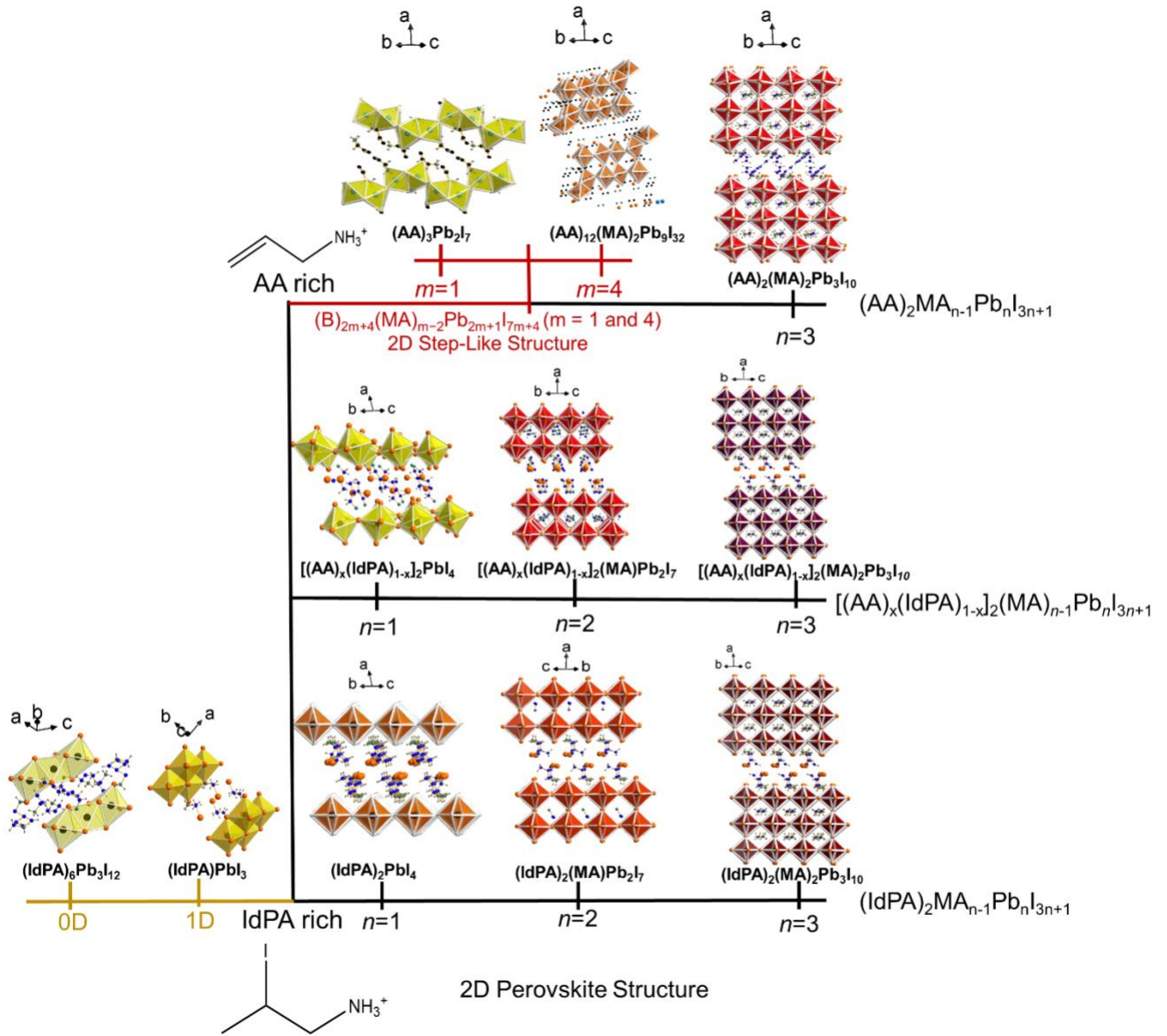
Figure 1. Structural overview of newly reported series of (100) lead iodide perovskites: (\text{AA})_2\text{MA}_{n-1}\text{Pb}_n\text{I}_{3n+1} ( n=3-4 ), [(\text{AA})_x(\text{IdPA})_{1-x}]_2\text{MA}_{n-1}\text{Pb}_n\text{I}_{3n+1} and (\text{IdPA})_2\text{MA}_{n-1}\text{Pb}_n\text{I}_{3n+1} ( n=1-4 ), as well as their perovskite-related substructures: (\text{AA})_2\text{Pb}_2\text{I}_7 , (\text{AA})_{12}(\text{MA})_2\text{Pb}_9\text{I}_{32} , (\text{IdPA})\text{PbI}_3 and (\text{IdPA})_6\text{Pb}_3\text{I}_{12} .
