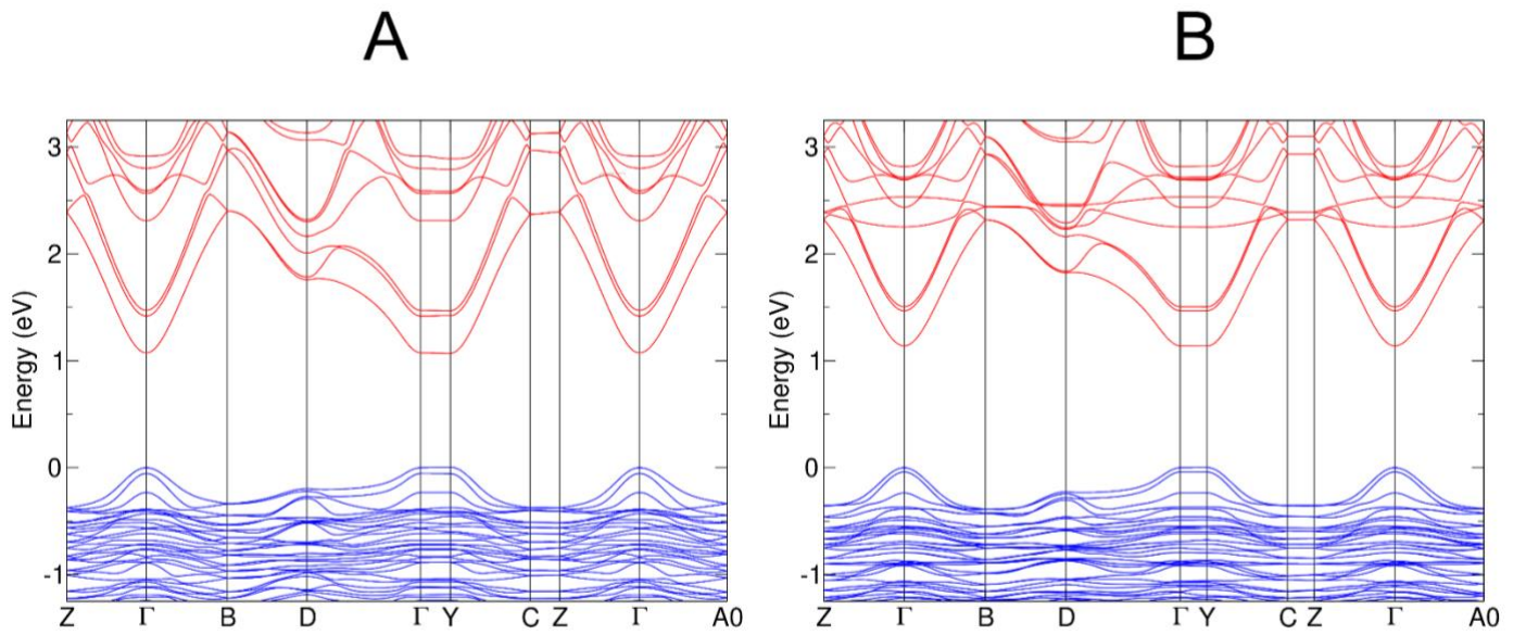
Figure 8. Computed band structures for (A) (\text{AA})_2\text{MA}_2\text{Pb}_3\text{I}_{10} and (B) (\text{IdPA})_2\text{MA}_2\text{Pb}_3\text{I}_{10} .
