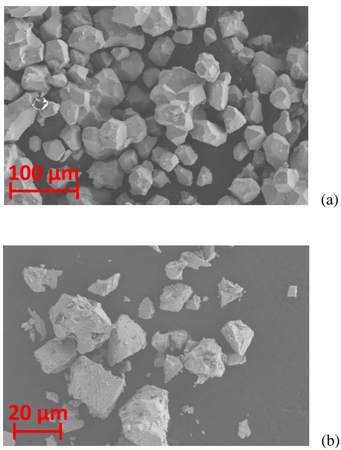
Figure 2 SEM images of ZSb01_2 (a) and ZP01_2 (b) doped with 1% Zn_3Sb_2 and 1% Zn_3P_2 , respectively.
