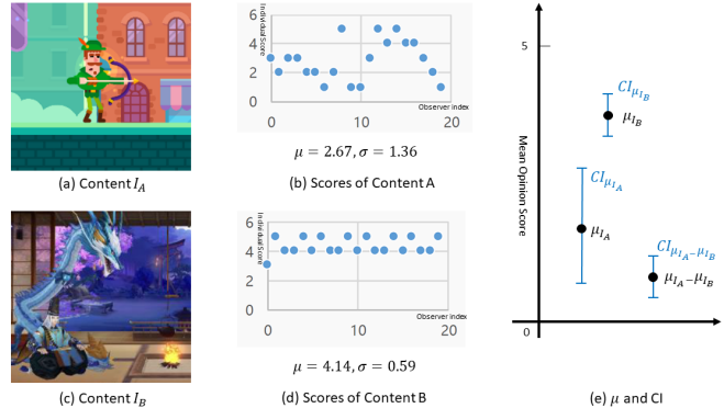
Fig. 1. Example of contents that have significantly different standard deviation \sigma , and demonstration of how Confidence Intervals (CI) could help to rank the aesthetic scores.
