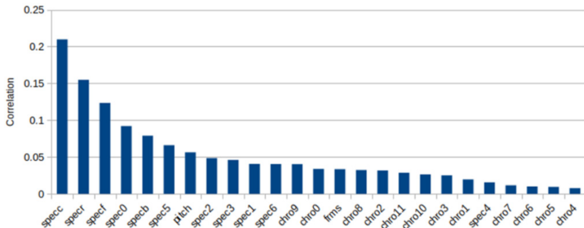
Figure 6. Correlation between 25 parameters and accuracy recognition. specc : spectral centroid, specr : spectral rolloff, specf : spectral flatness, specb : spectral bandwidth, spec0-6 : spectral contrast, chro0-11 : chroma, frms : root-mean-square (RMS) value calculated for each frame.
