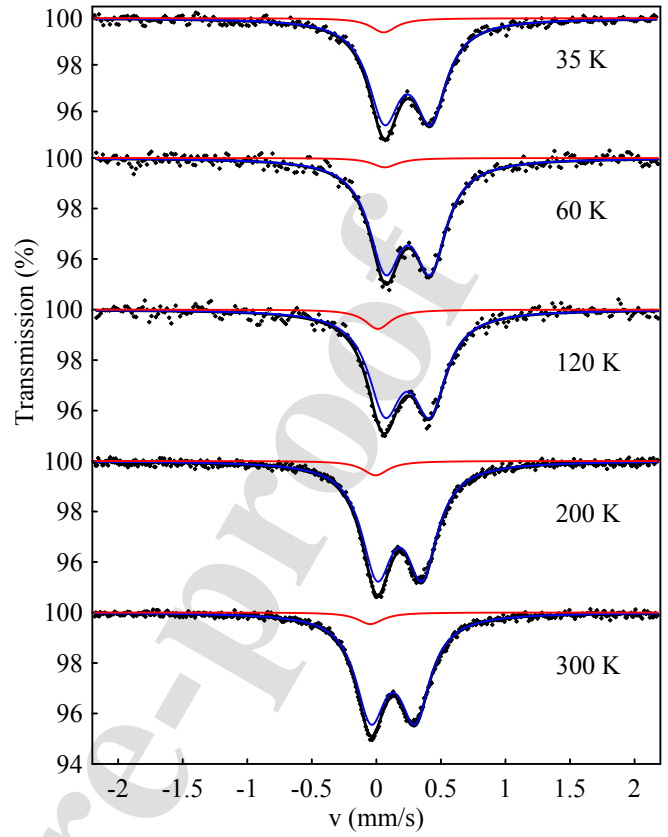
Figure 3: TMS spectra of \text{UFe}_{0.40}\text{Ge}_2 measured at several temperatures from the range 35–300 K and in zero applied magnetic field, fitted by a sum (black curve) of one doublet and one singlet component (blue and red lines, respectively). For details of the fits see the text.
