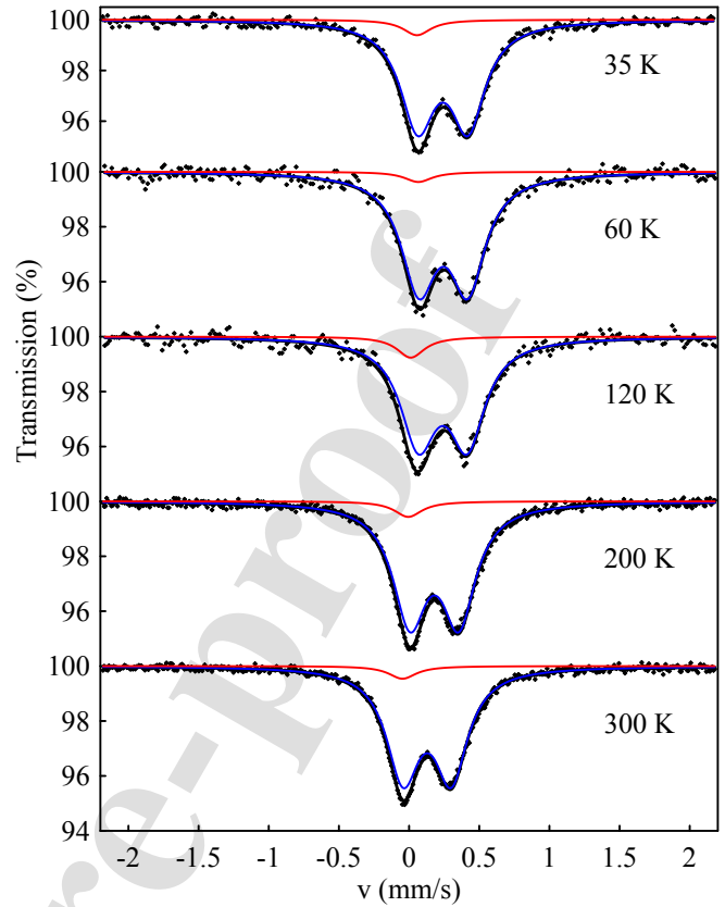
Figure 3: TMS spectra of \text{UFe}_{0.40}\text{Ge}_2 measured at several temperatures from the range 35–300 K and in zero applied magnetic field, fitted by a sum (black curve) of one doublet and one singlet component (blue and red lines, respectively). For details of the fits see the text.
