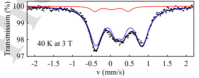
Figure 6: TMS spectrum of \text{UFe}_{0.40}\text{Ge}_2 measured at 40 K and in external magnetic field of 3 T.
