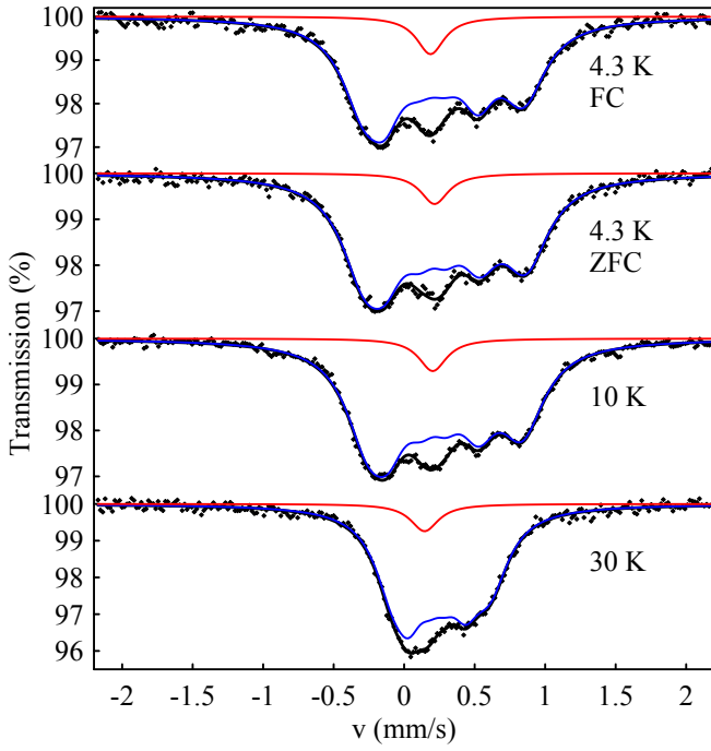
Figure 4: TMS data collected for \text{UFe}_{0.40}\text{Ge}_2 at several temperatures from the magnetically ordered region and in zero applied magnetic field, fitted by a sum (black line) of one sextet and one singlet component (blue and red curves, respectively). FC marks the spectrum measured in zero magnetic field, after cooling the sample in the field of 3 T. For details of the fits see the text.
