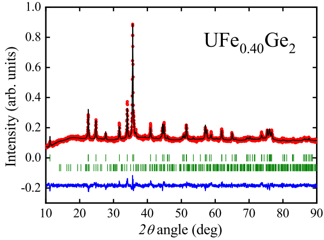
Figure 1: Powder X-ray diffraction pattern of \text{UFe}_{0.40}\text{Ge}_2 (red circles) plotted along with results of the Rietveld refinement of its crystal structure (black curve). Upper and lower green ticks indicate Bragg positions for the major ( \text{UFe}_{0.40}\text{Ge}_2 ) and the impurity ( \text{U}_9\text{Fe}_7\text{Ge}_{24} ) phases, respectively. Blue curve shows the difference between the experimental and the theoretical patterns.
