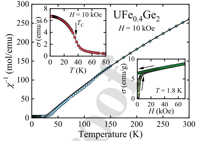
Figure 2: Temperature dependence of inverse magnetic susceptibility \chi^{-1} of \text{UFe}_{0.40}\text{Ge}_2 ; solid line is a fit of the modified Curie-Weiss law to the experimental data (for details see the text). Upper inset: low temperature variation of mass magnetization \sigma measured in field-cooling regime; an arrow marks the ferromagnetic ordering temperature T_C . Lower inset: \sigma as a function of increasing (open symbols) and decreasing (closed symbols) applied magnetic field H .
