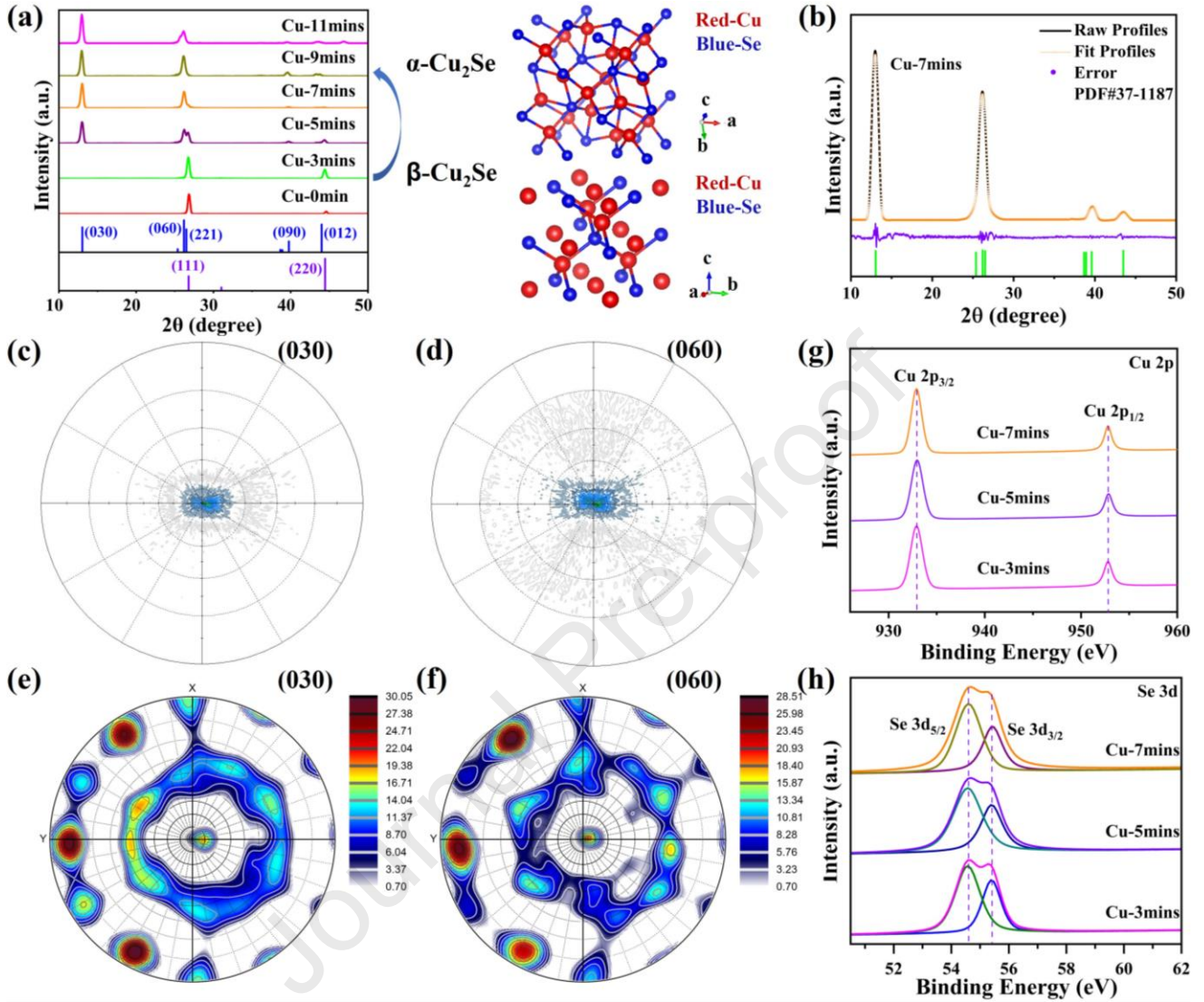
Fig.1. (a) XRD patterns of thin films with different composition ratios at the same heat treatment temperature. (b) XRD refinement of Cu-7mins. (c) 2\theta = 13.039^\circ and (d) 2\theta = 26.188^\circ X-ray pole figure XRD pole figures of Cu-7mins.; XRD polar figures of (e) 2\theta = 13.039^\circ and (f) 2\theta = 26.188^\circ after ATEX (Analysis Tools for Electron and X-ray diffraction) analysis. (g) XPS spectra of Cu in Cu-3mins, Cu-5mins and Cu-7mins thin films. (h) XPS spectra of Se in Cu-3mins, Cu-5mins and Cu-7mins thin films.
