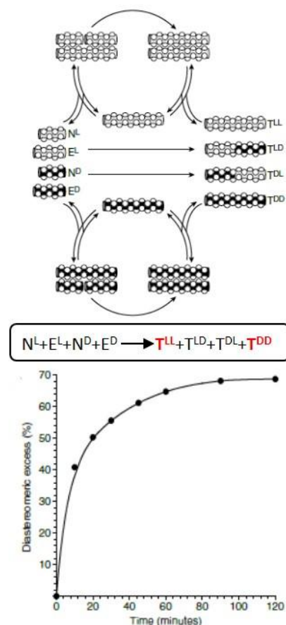
Figure 22 Top: schematic representation of the stereoselective replication of peptide residues with the same handedness. Below: diastereomeric excess ( de ) as a function of time. de (\%) = [(T^L + T^{DD}) - (T^D + T^{LL})] / T^{\text{total}} . Adapted from reference 539 with permission from Nature publishing group.
