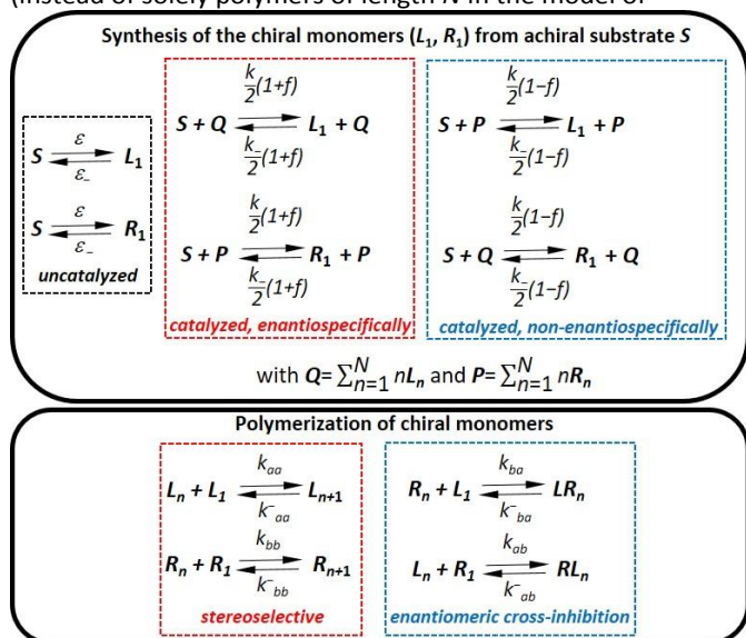
Figure 25 Hochberg model for chiral polymerization in closed systems. N = maximum chain length of the polymer, f = fidelity of the feedback mechanism, Q and P are the total concentrations of left -handed and right -handed polymers, respectively. \varepsilon ( \varepsilon_+ ), k ( k_+ ), k_{aa} ( k_{aa} ), k_{bb} ( k_{bb} ), k_{ba} ( k_{ba} ), k_{ab} ( k_{ab} ) denote the forward (reverse) reaction rate constants. Adapted from reference 575 with permission from the Royal Society of Chemistry.
