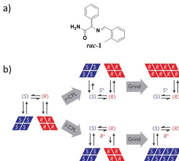
Figure 16 a) Molecular structure of rac -1. b) CPL-controlled complete attrition-enhanced deracemization of rac -1. (S) and (R) are the enantiomers of rac -1 and S* and R* are chiral photoproducts formed upon CPL irradiation of rac -1. Reprinted from reference 419 with permission from Nature publishing group.
