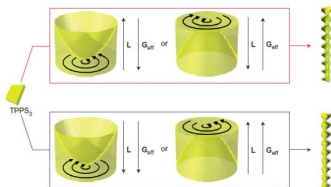
Figure 5 Control of the handedness of TPPS 3 helical assemblies by the relative orientation of the angular momentum of the rotation (L) and the effective gravity (G eff ). TPPS 3 : tris-(4-sulfonatophenyl)phenyl porphyrin. Reprinted from reference 161 with permission from Nature publishing group.
