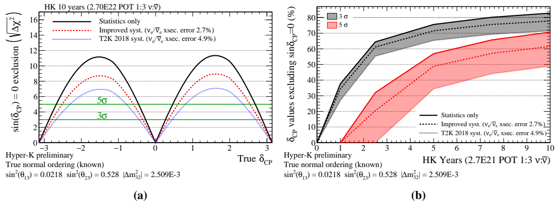
Figure 1: (a) Sensitivity to exclude CP violation as a function of the true value of \delta_{CP} . The solid black line shows the case where no systematics are considered (statistics only), the dotted red line represents the Hyper-K improved model and the dashed blue line shows the T2K 2018 model. (b) Percentage of \delta_{CP} values excluding \sin\delta_{CP} = 0 at 3\sigma (black) and 5\sigma (red) significance, as a function of accumulated Hyper-K data. The line styles represent different systematic models.
