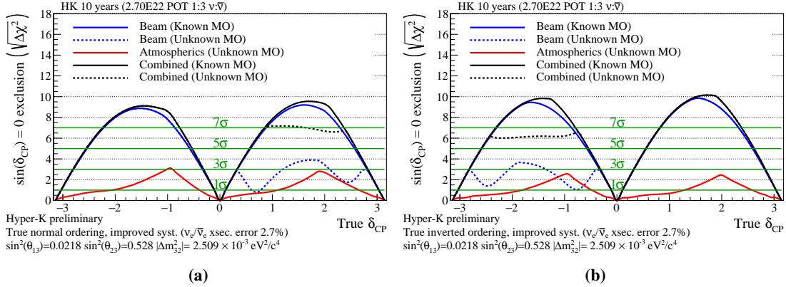
Figure 2: Sensitivity to exclude CP violation using beam neutrinos (blue), atmospheric neutrinos (red) and the combination of the two (black). Solid (dashed) lines indicate that the MO is known (unknown). (a) Assuming true NO. (b) Assuming true IO.
