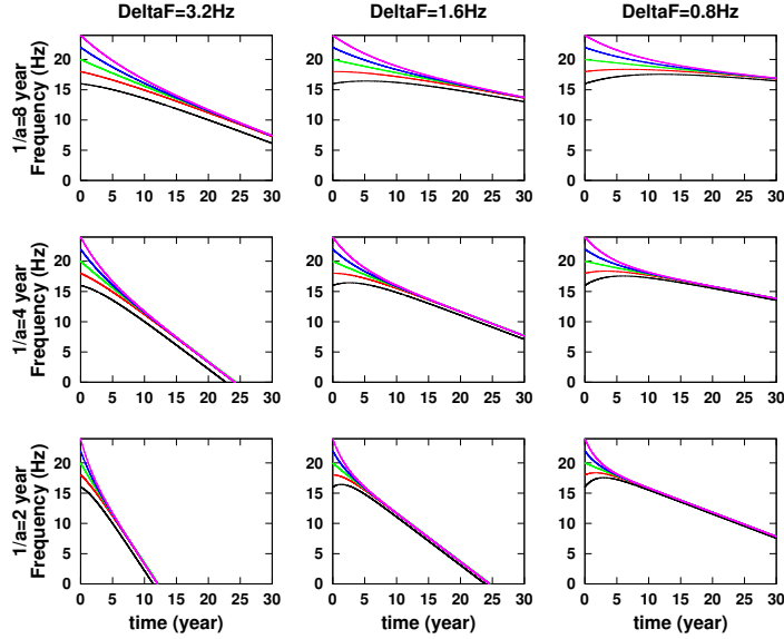
Figure 1: Examples of frequency decline for 5 whales, from the simple model given by equation (1). Initial values F_i(0) are chosen as 16 Hz, 18 Hz, 20 Hz, 22 Hz and 24 Hz to represent plausible values for blue whales. Parameters a and \overline{\Delta F} vary to show distinct behaviours, a being constant for each line and \overline{\Delta F} for each column. Individual \Delta F_i are randomly chosen with a Gaussian probability function with standard deviation \sigma_{\Delta F} = 0.3 Hz and mean value \Delta F as shown in each column.
