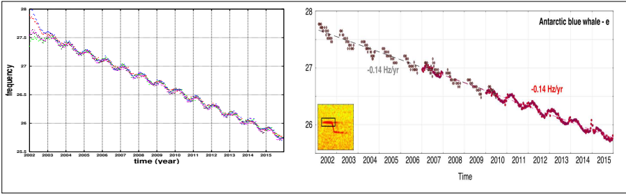
Figure 5: Left : result of the modelling of the frequency variations of the unit A of the Antarctic blue whales song. Parameters of the model : n = 10 whales (of which only 5 are represented for clarity), initial average frequency \overline{F_0} = 27.7 Hz, with a standard deviation of \sigma_{F_0} = 0.08 Hz, \overline{\Delta F_{(a)}} = 0.076 Hz, \sigma_{\Delta F_{(a)}} = 0.01 Hz, \overline{\Delta F_{(b)}} = 0.22 Hz, \sigma_{\Delta F_{(b)}} = 0.05 Hz, a = 1.825 \text{ yr}^{-1} and \phi = 2.9 radians. A random noise has been added to the data, with a zero average and a 0.02 Hz standard deviation. Right : data of the frequency variation obtained by [Leroy et al., 2018a].
