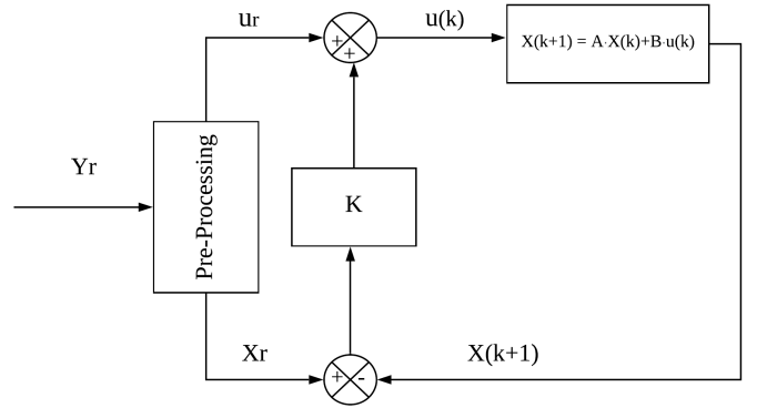
Fig. 4: Modified LQR Control problem
