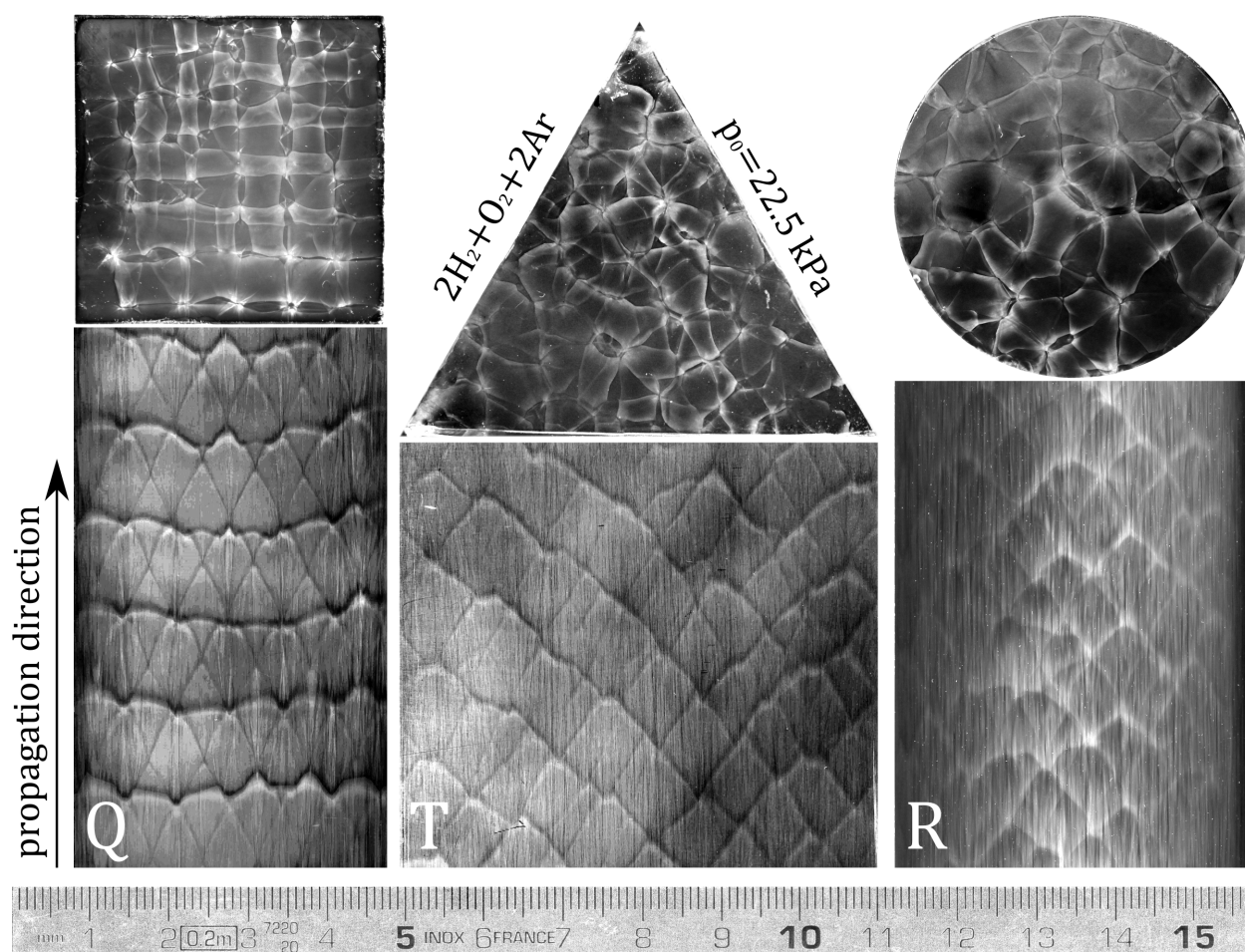
Figure 5: Front-view (top) and longitudinal (bottom) soot recordings in the mixture 2\text{H}_2 + \text{O}_2 + 2\text{Ar} at p_0 = 22.5 \text{ kPa} in round (R), triangular (T) and square (Q) tubes with the same cross-section area ( 16 \text{ cm}^2 ).
