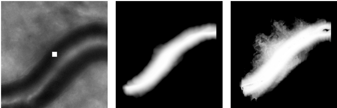
Figure 13: Left: Crop of the input image of Figure 7, with a pixel i marked as the centre of the white square. Centre: Neighbourhood \mathcal{N}_i^k in the non binary-weighted co-circularity graph with k = 15 and parameters \sigma = 5 , p = 7 and \beta = \frac{\pi}{6} . Right: Neighbourhood of the same pixel in the non binary-weighted graph with same parameters except \sigma = 2 . As we can see the two neighbourhoods are not ordered and the one for \sigma = 2 is less accurate with respect to the underlying vessel shape.
