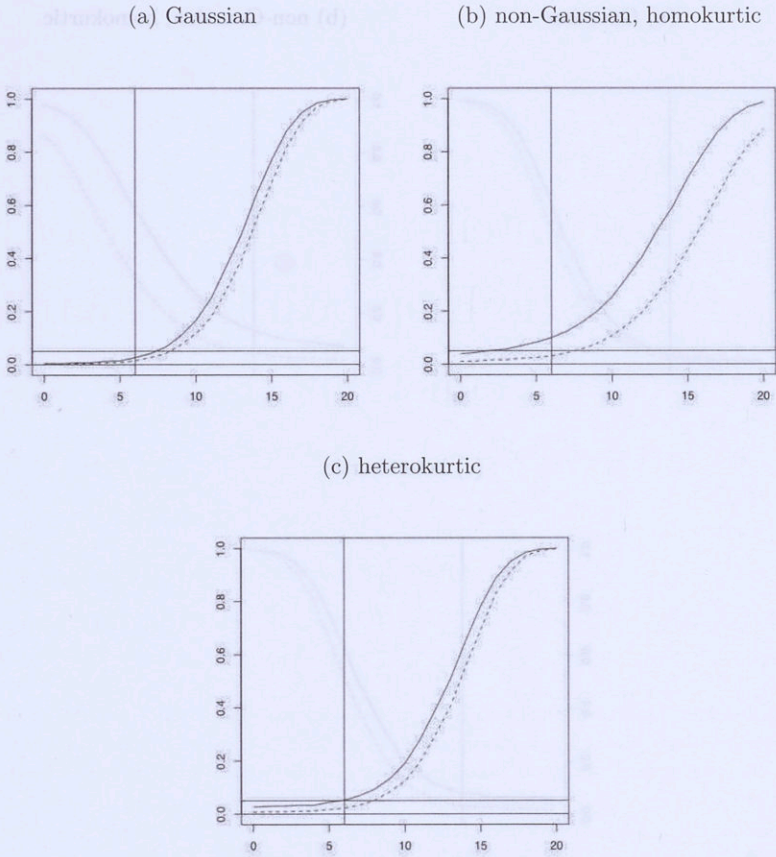
Figure 3: Rejection frequencies (out of N = 10,000 replications), in Experiment 3 (see Section 5), of Flury's Gaussian test \phi_{\text{Flury}}^{(n)} (solid line) and our pseudo-Gaussian test \phi_{\dagger}^{(n)} (dotted line). The asymptotic nominal size is \alpha = 5\% ; k = 2 , m = 2 , q = 1 . Sample sizes are n_1 = n_2 = 100 .
