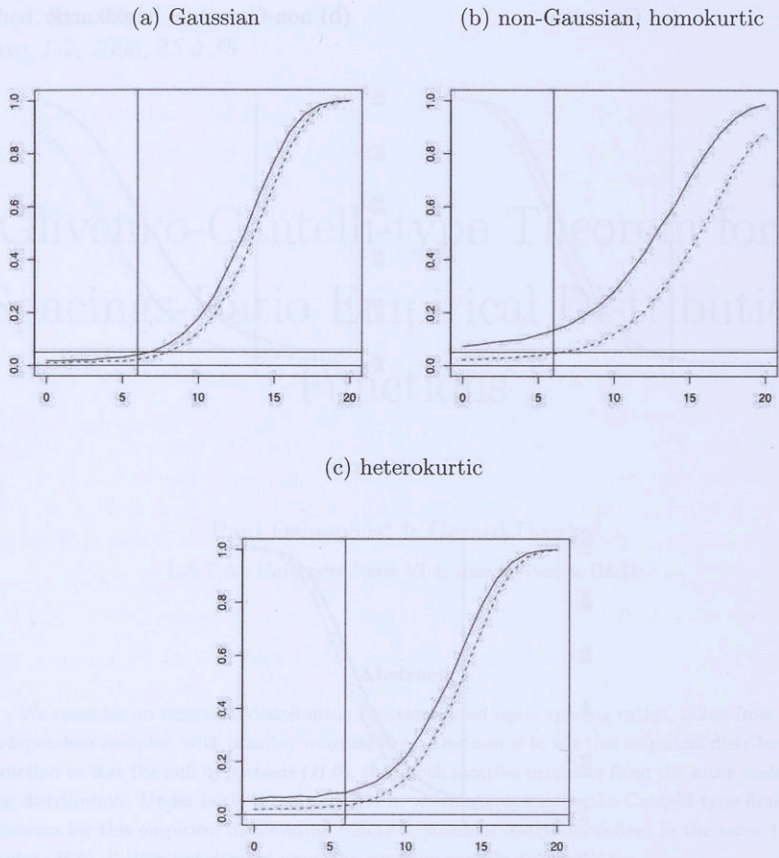
Figure 2: Rejection frequencies (out of N = 10,000 replications), in Experiment 2 (see Section 5), of Flury's Gaussian test \phi_{\text{Flury}}^{(n)} (solid line) and our pseudo-Gaussian test \phi_{\dagger}^{(n)} (dotted line). The asymptotic nominal size is \alpha = 5\% ; k = 2 , m = 2 , q = 1 . Sample sizes are n_1 = n_2 = 100 .
