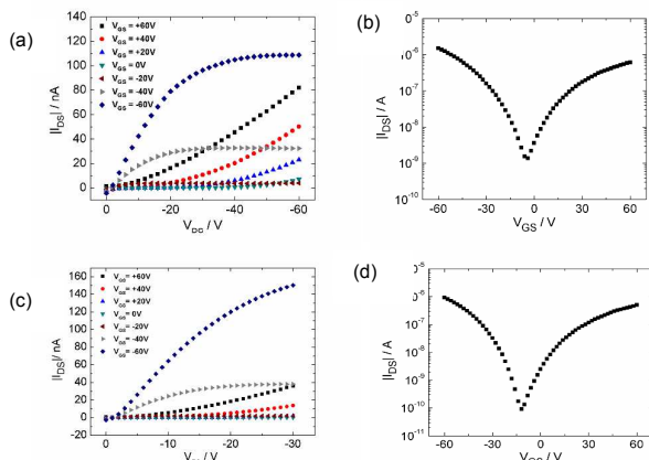
Figure 6. Output (a) and transfer (b) characteristics of compound 4a . Output (c) and transfer (d) characteristics of compound 4b . [ W = 10\text{mm} , L = 20\ \mu\text{m} ] [ V_{DS} = -30\text{V} in the transfer curves]
