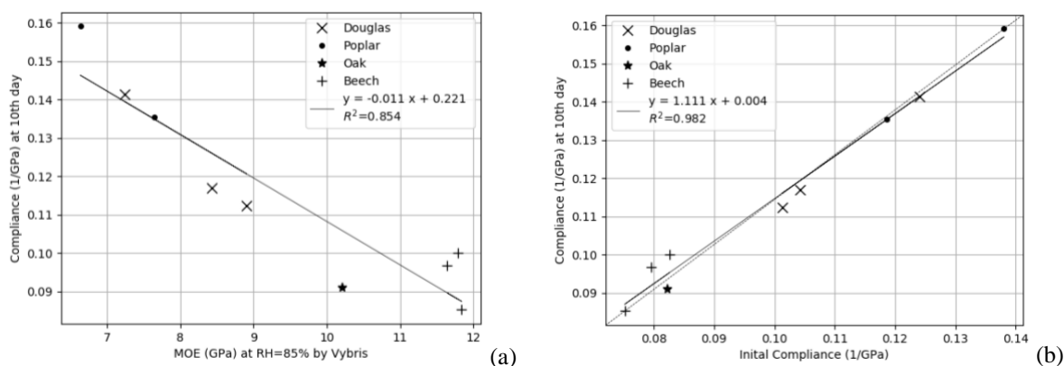
Figure 7: The comparison of creep test result
