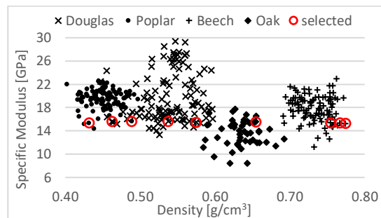
Figure 2: Preliminary measurements of vibrational specific modulus and density on all specimens and sampling results for a fixed domain of specific modulus.
