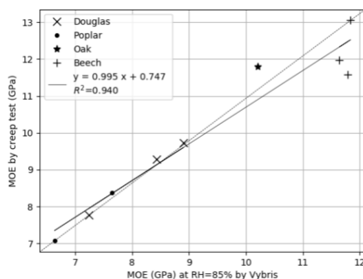
Figure 5: MOE by different testing method.
