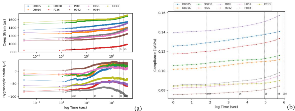
Figure 6: the 10-day creep test result
