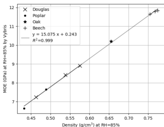
Figure 4: Relationship between density and MOE.
