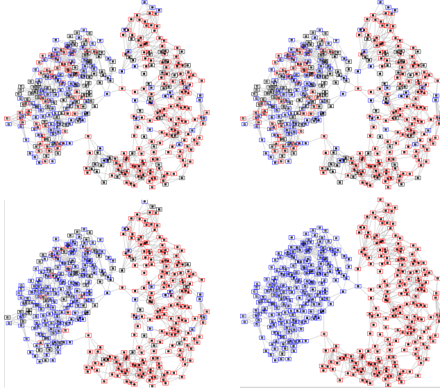
Figure 7: Application of the level set active contours to data clustering. The graph is built from a subset of the MNIST database, as a k -NNG with k = 5 . The similarity function is computed using two-sided tangent distance and the velocity is defined according to (6.9) where F as in the Chan-Vese model. Each cluster is represented by a front, randomly initialized.
