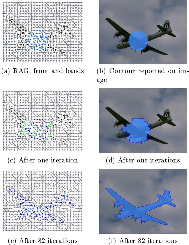
Figure 6: Illustration of active contours on a RAGG. The RAG is built from a superpixel decomposition of the initial image, where each region is connected to its adjacent regions. The weight and velocity functions are computed from the mean color inside regions. Left column shows the RAG, with the propagating front in blue and candidate bands in red (inner) and green (outer). Right column shows the initial image with the propagating front transposed from the RAG (using the boundaries of the superpixels).
