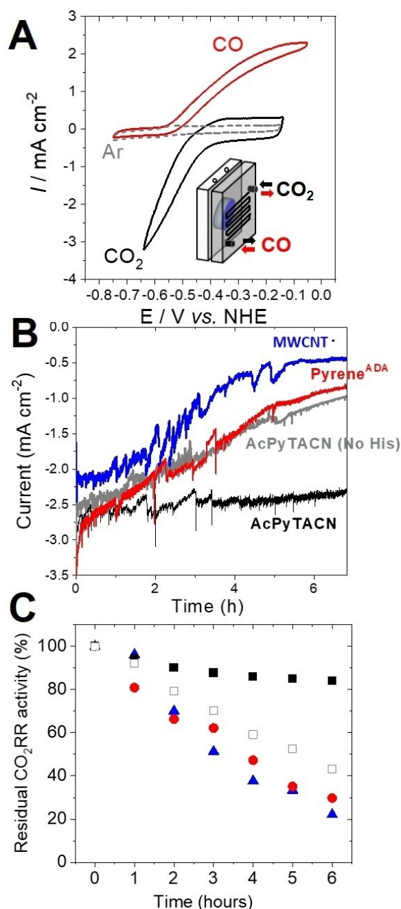
Figure 5. A) CVs of the Rec-RrCODH His -functionalized Ni-TACN-modified gas-diffusion bioelectrode under Ar, CO and \text{CO}_2 (50 mM Tris-HCl, pH 8.5, \nu = 5 \text{ mV s}^{-1} ). (inset) Schematic representation of the gas-diffusion electrochemical cell. B) Chronoamperometry performed at -0.76 \text{ V} vs. NHE under \text{CO}_2 for 6 hours under \text{CO}_2 for (grey) Rec-RrCODH His immobilized at nonmodified MWCNT electrode, (red) Rec-RrCODH His immobilized at pyrene ADA -modified MWCNT electrode, (blue) Rec-RrCODH immobilized at AcPyTACN-modified MWCNT electrode and (black) His-tagged Rec-RrCODH immobilized at AcPyTACN-modified MWCNT electrode. C) Residual \text{CO}_2\text{RR} activity (%) measured each hour for (▲) Rec-RrCODH His immobilized at nonmodified MWCNT electrode, (●) Rec-RrCODH His immobilized at pyrene ADA -modified MWCNT electrode, (□) Rec-RrCODH immobilized at AcPyTACN-modified MWCNT electrode and (■) Rec-RrCODH His immobilized at AcPyTACN-modified MWCNT electrode.
