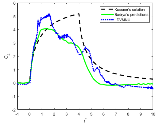
Figure 9: LDVMNU prediction of the encounter of a gust of length D = 4 compared with simulations from [1] and reference theory
