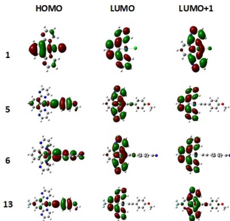
Fig. 11 The frontier orbitals of complexes 1 , 5 , 6 and 13 .
