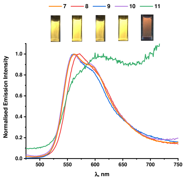
Fig. 8 Normalized emission spectra of alkyl-platinum complexes 7-11 in deoxygenated \text{CH}_2\text{Cl}_2 solution ( c \sim 10^{-5} M). \lambda_{\text{exc}} = \lambda_{\text{max}}^{\text{abs}} of the lowest energy band Inset: picture of \text{CH}_2\text{Cl}_2 solution taken under UV irradiation
