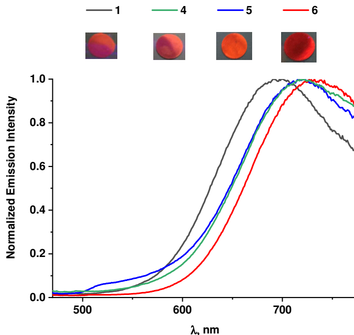
Fig. 9 Normalized emission spectra of complexes 1 , and 4-6 in KBr matrix (2 w%). \lambda_{\text{exc}} = \lambda_{\text{max}}^{\text{abs}} of the lowest energy band in \text{CH}_2\text{Cl}_2 solution Inset: picture of KBr pellets taken under UV irradiation.
