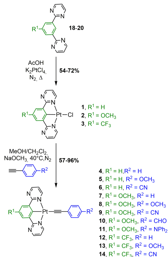
Scheme 1 Synthesis of N ^C^ N cyclometalated chloro-platinum(II) complexes 1-3 and alkynyl-platinum(II) complexes 4-14 .
