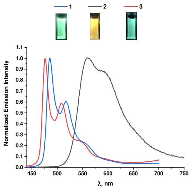
Fig. 7 Normalized emission spectra of chloro-platinum complexes 1-3 in deoxygenated CH 2 Cl 2 solution ( c \sim 10^{-5} M). \lambda_{\text{exc}} = \lambda_{\text{max}}^{\text{abs}} of the lowest energy band Inset: picture of CH 2 Cl 2 solution taken under UV irradiation
