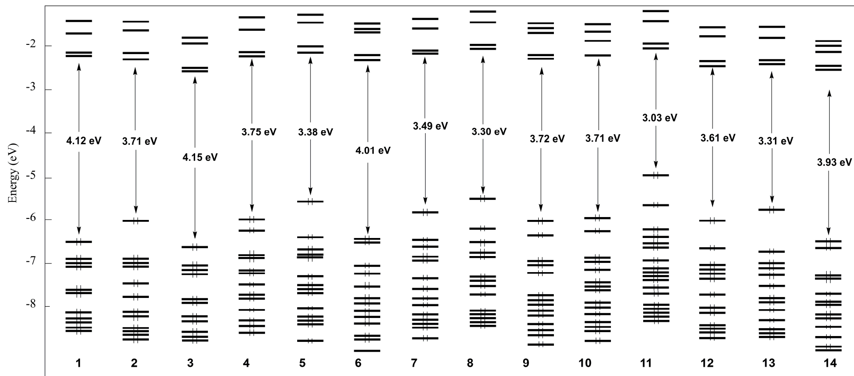
Fig. 10 Kohn-Sham MO diagrams of complexes 1-14 .
