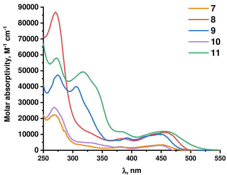
Fig. 6 Absorption spectra of alkynyl-platinum complexes 7-11 in CH 2 Cl 2 ( c \sim 10^{-5} M)
