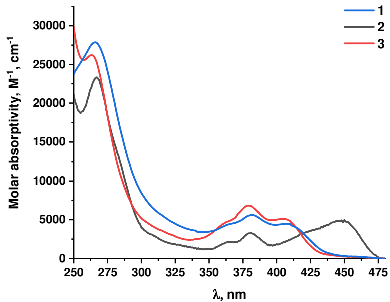
Fig. 5 Absorption spectra of chloro-platinum complexes 1-3 in CH 2 Cl 2 ( c \sim 10^{-5} M)
