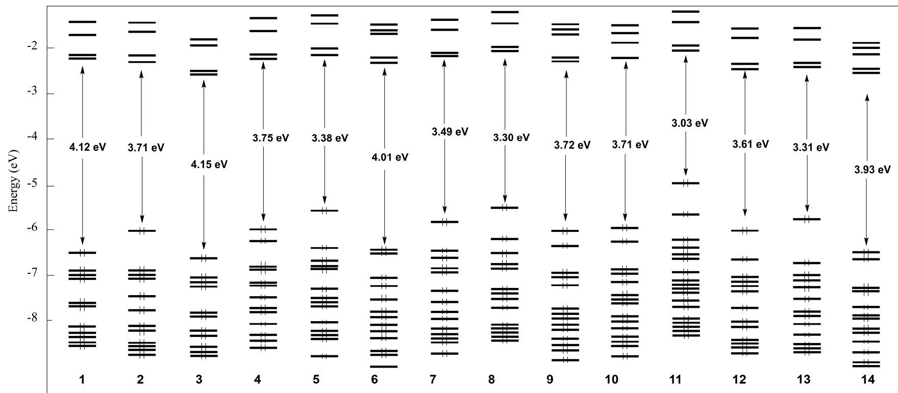
Fig. 10 Kohn-Sham MO diagrams of complexes 1-14 .
