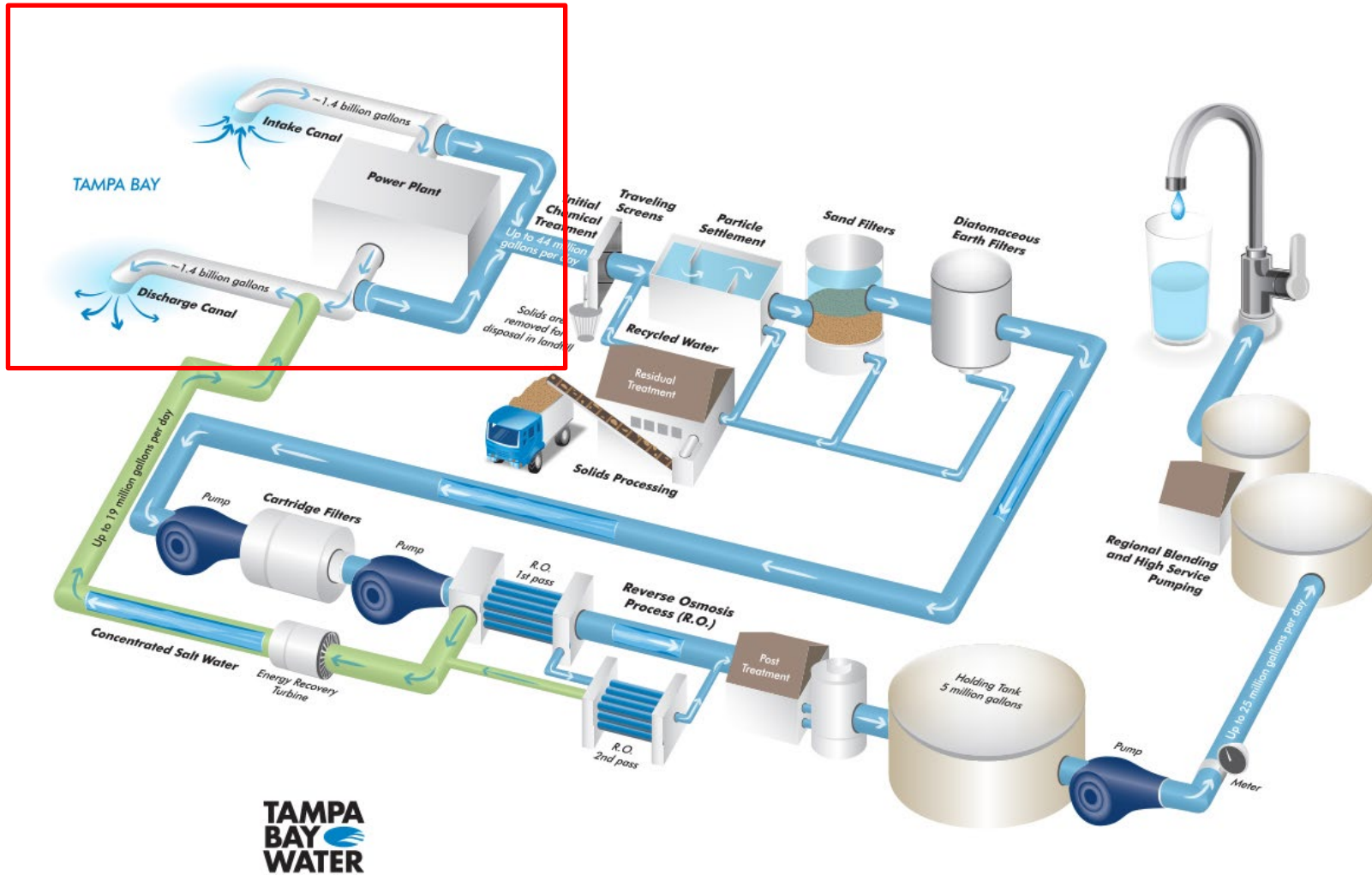
Tampa Bay Seawater Desalination Plant Process Diagram
