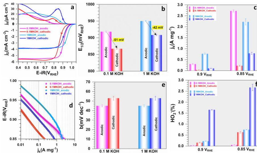
Figure 3. Scan direction effect. (a) LSV (1600 rpm, 5 \text{ mV s}^{-1} ) of ORR at an RRDE: disk (bottom) and ring (top). (b) Half-wave potential. (c) Kinetic current density. (d) Tafel plots. (e) Tafel slope. (f) Incomplete hydroperoxide anion. Error bars represent 1 SD ( n \geq 3 ).
