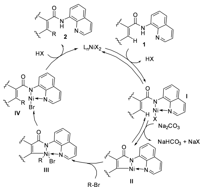
Scheme 2. Proposed mechanistic pathway.
