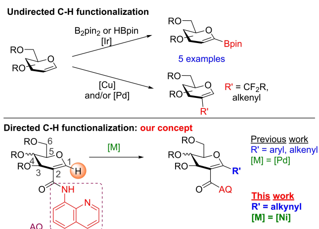
Scheme 1. The proposed methodology versus previous works on C–H functionalization of glycols.
