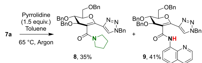
Scheme 3. Removal of the directing group.
