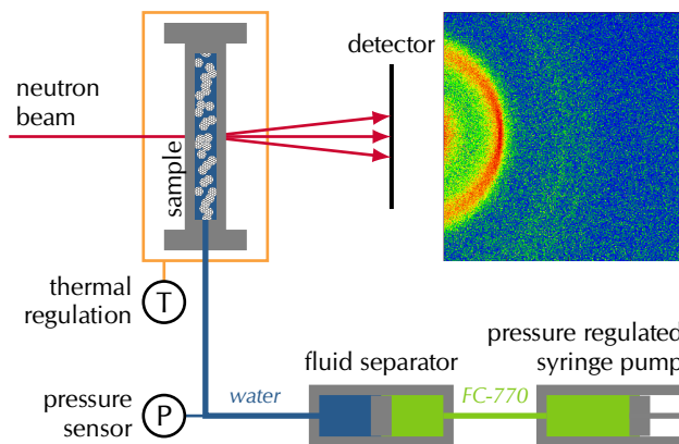
Figure 3: Schematic of the setup used for the study of the deformation of hydrophobized MCM-41 nanopores when performing an intrusion/extrusion isotherm. Inset: Typical 2D small-angle diffraction pattern obtained after calibration and instrument correction.
