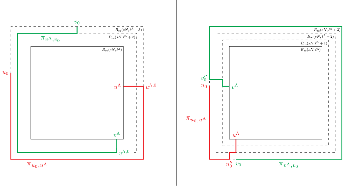
Figure 6: Example of the construction of the portion of \pi which is contained in B_\infty(sN, \ell^\Lambda + 3) \setminus B_\infty(sN, \ell^\Lambda) in dimension 2. On the left, this is an example of the case where \|u_0 - v^\Lambda\|_1 > 3 or \|v_0 - u^\Lambda\|_1 > 3 and on the right the other case.
