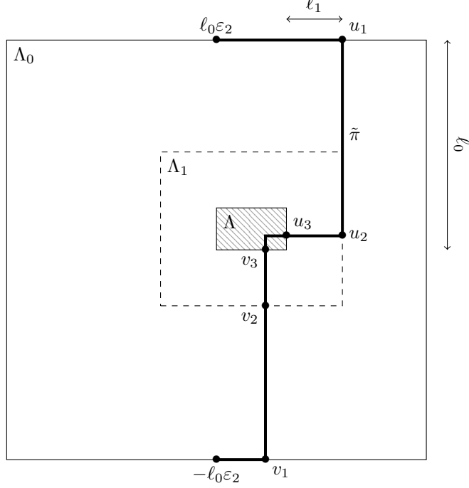
Figure 7: Example of the construction of \tilde{\pi} in an overlapping pattern in dimension 2.
