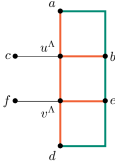
Figure 1: Example of a pattern which can not be taken by a geodesic. The passage times of the edges in red are equal to 4 and those of the edges in green are equal to 1.
