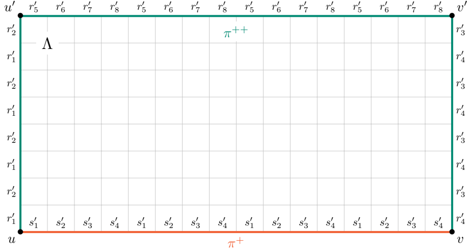
Figure 5: Paths \pi^+ and \pi^{++} with their passage times in the pattern for the proof of Theorem 1.8 in the bounded case with d = 2 , k = 4 , \ell = 2 and \alpha = 4 .
