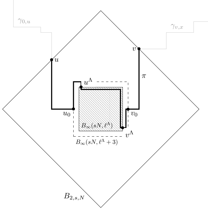
Figure 2: Example of the construction of \pi in dimension 2.
