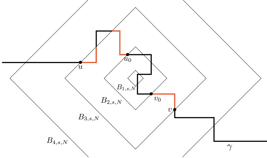
Figure 3: Elements involved in the first modification. The edges whose time can be modified by the first modification are represented in red.
