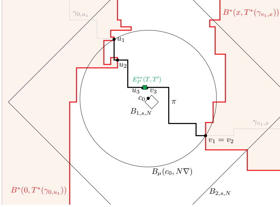
Figure 4: The construction of \pi , of the vertices u_1, u_2, u_3, v_1, v_2, v_3 and of the pattern-location in dimension 2.
