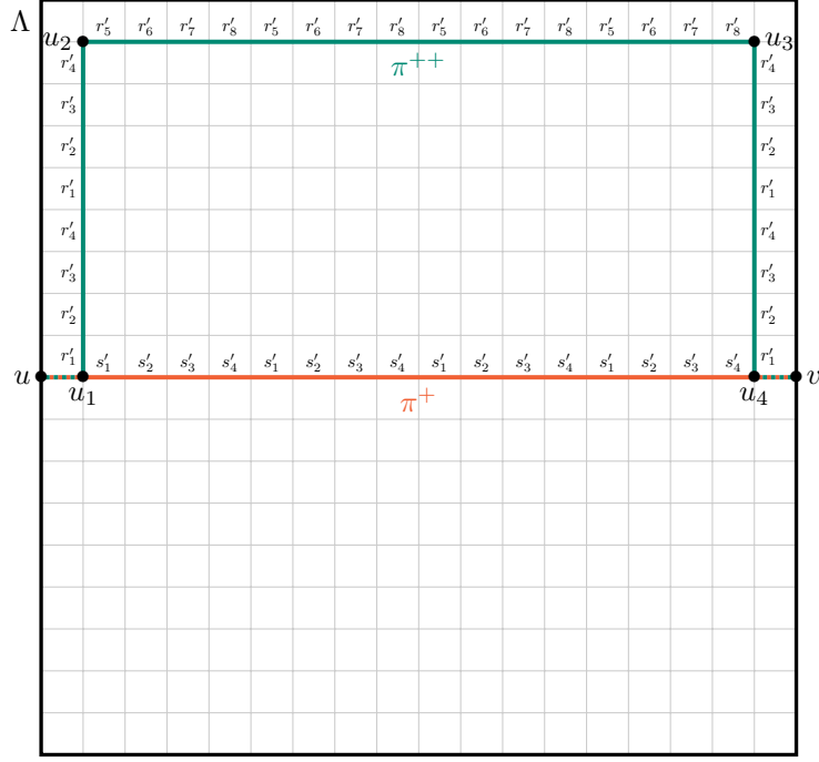
Figure 1: Paths \pi^+ and \pi^{++} with their passage times in the pattern for the proof of Theorem 1.7 in the bounded case with d = 2 , k = 4 , \ell = 2 and \alpha = 4 .
