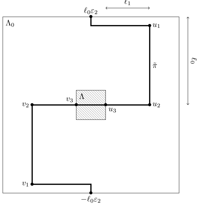
Figure 6: Example of the construction of \tilde{\pi} in an overlapping pattern in dimension 2.
