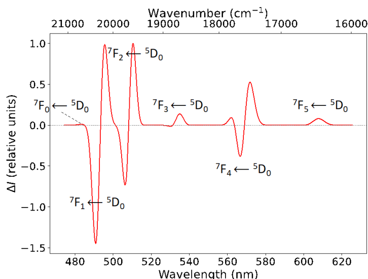
Figure 8. Calculated CPL spectrum of [\text{Eu}(\text{tta})_3(\mathbf{6M})] complex in relative units. The Gaussian broadening was performed with a \sigma value of 10 meV. No spectral shift has been applied.
