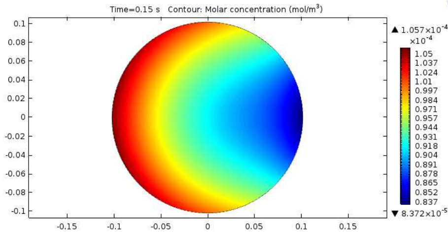
Figure 1: Snapshots of the molar concentration profile of TMA on the substrate surface for 150 ms after the beginning of the TMA pulse (the loading door is located at the right part of the wafer)
