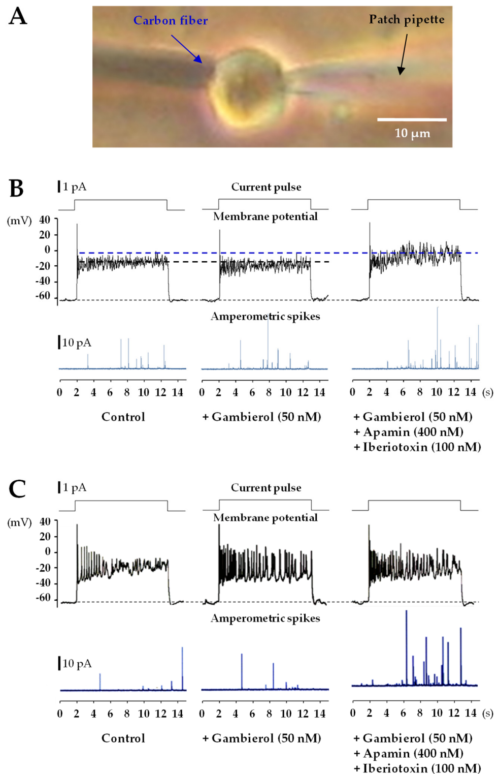
Figure 5. Combined whole-cell current-clamp and amperometric recordings in single fetal AMC cells under control conditions, and during the action of gambierol and K_{Ca} blockers. (A) Microphotograph of a typical recording configuration for single-cell amperometry, using a polarized carbon fiber electrode to detect exocytotic events, related to catecholamine release, and a whole-cell current-clamp pipette to control the level of membrane depolarization imposed to the cell membrane. (B,C) Whole-cell current-clamp recordings showing in the upper tracing the current
