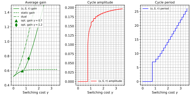
Fig. 4: Evolution of the optimal (s, S, \tau) -cycle for a range of switching cost values
