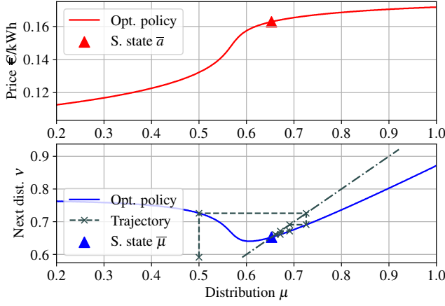
(c) Optimal decision for the long-run average reward (provider action and next customer distribution) for low switching cost. Graphical iteration is drawn in dotted lines.
