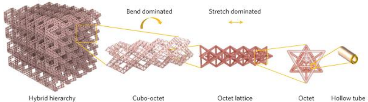
Fig. 24. An example of a hierarchical lattice structure. Note that every next tier in the hierarchy can be associated with a higher level of detail. Permission to reprint from Springer Nature copyright 2016 [173].
