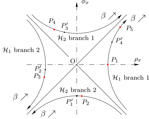
Figure 5: Case -1 < J < 0 . Fractional parameter \alpha = \pi/2 + i\beta ( \beta > 0 ). The sequence of points P_i is analyzed in the text. If d_i = OP_i , sequences (d_{2i}) and (d_{2i+1}) are diverging. The corresponding resonator is unstable.
