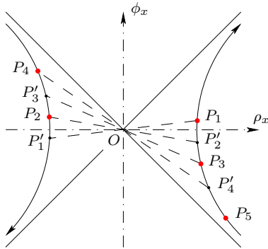
Figure 4: The case J = J' < -1 , \beta > 0 and \mathfrak{s} = -1 . Points P_i are defined as in Fig. 3. Point P'_i is deduced from P_i in a \pi -rotation, and P_{i+1} is deduced from P'_i in a hyperbolic rotation of angle -\beta . If d_i = OP_i , the sequences (d_{2i}) and (d_{2i+1}) are diverging. The resonator is unstable.
