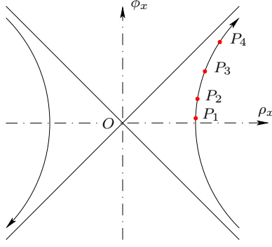
Figure 3: A sequence (P_i) for J = J' < -1 , \beta > 0 and \mathfrak{s} = 1 . The values taken at points P_1, P_3, P_5 etc. by the Wigner distribution on \mathcal{M}_1 are equal. They are also equal to the values of the Wigner distribution on \mathcal{M}_2 taken at points P_2, P_4 , etc. Point P_{i+1} is deduced from P_i in a hyperbolic rotation of angle \beta . If d_i = OP_i , both sequences (d_{2i}) and (d_{2i+1}) are diverging, which shows that the Wigner distribution on each mirror spreads over an increasingly wide area after every reflection: the resonator is unstable.
