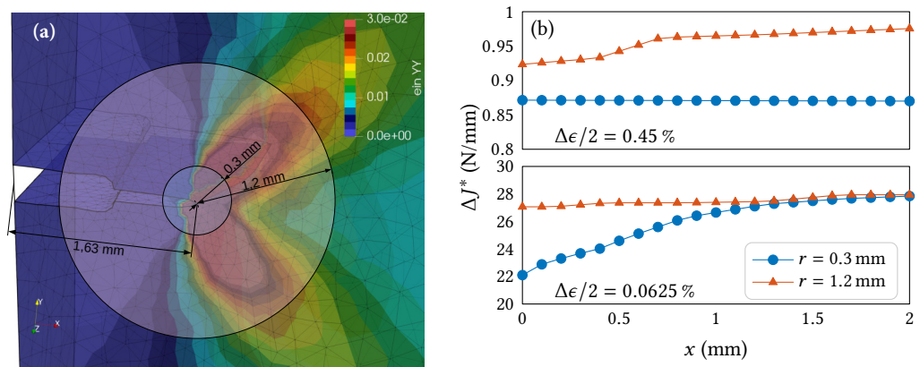
Figure A.1 Dependency of \Delta J^* to the chosen domain size a for loading corresponding to \Delta\epsilon/2 = 0.45\% : (a) surface representation of the chosen domain radius; (b) \Delta J^* for two domains and two loads; x describes the location along the crack front, x = 0 corresponds to the free surface.
