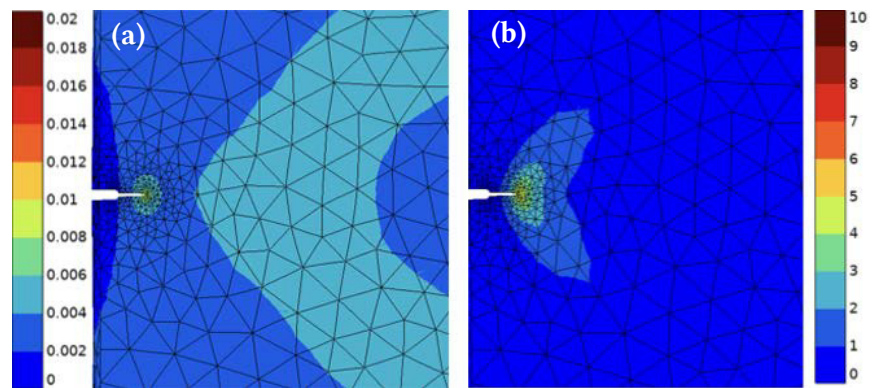
Figure 11 Strain energy density at maximum applied loading using direct non-local field where characteristic length is set to 400\ \mu\text{m} : (a) w_e and (b) w_p (values are divided by 10^6 for reading purpose), applied strain level corresponds to \Delta\epsilon/2 = 0.25\ \% .
