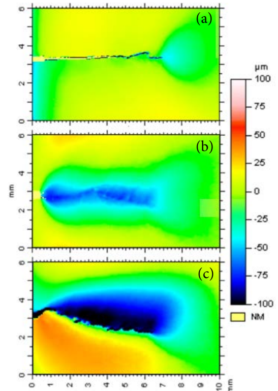
Figure 2 Measurements of surface roughness for (a) \Delta\epsilon/2 = 0.0625\% , (b) \Delta\epsilon/2 = 0.25\% and (c) \Delta\epsilon/2 = 0.45\% and R_\epsilon = 0 . Adapted from (Trabelsi 2019). SENT specimen corresponding to Figure 3.
