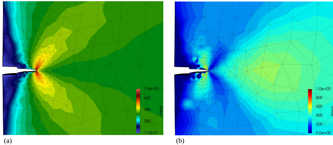
Figure 8: (a) Von Mises equivalent stress and (b) Trace of stress tensor \text{tr}(\sigma) for \Delta\varepsilon/2=0.375\% and R_\varepsilon=0
