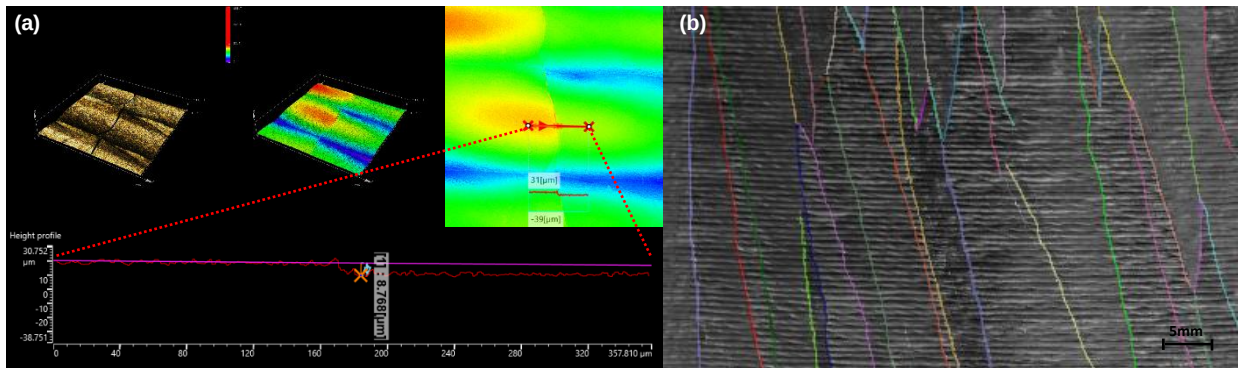
Figure 6: Laser confocal imaging of the grain boundary area. a. 3D optical image and contour map with the extracted cross-section height profile of grain boundary area. b. Grain boundary recognition under image segmentation.
