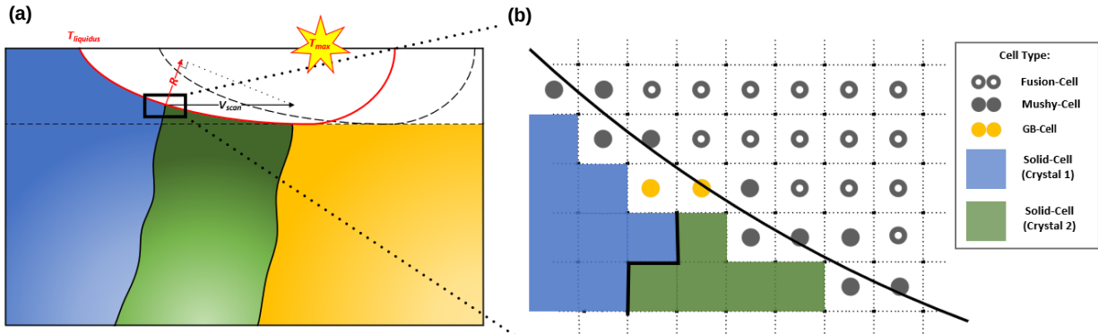
Figure 2: One timestep in the invasion model. a. Schematic of local solidification condition. b. Numerical representation of the simulation domain.
