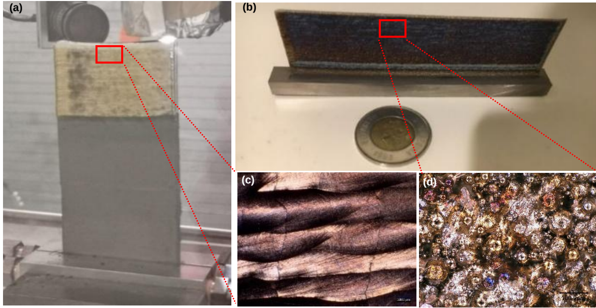
Figure 4: Building configuration and surface topology comparison of the wire (a, c) & powder (b, d) DED fabricated Ti-6Al-4V thin wall structures
