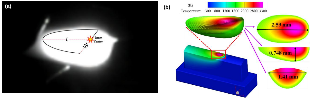
Figure 7: Melt pool geometry validation. a. High-speed imaging of transient melt pool geometry with L and W representing the length and width of the melt pool. b. Melt pool geometry extracted from the CFD simulation.
