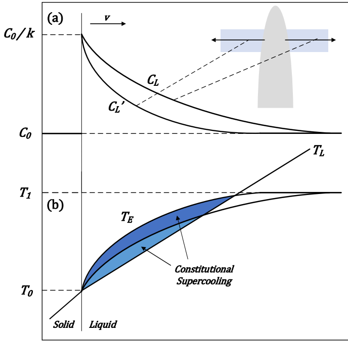
Figure 3: The origin of constitutional supercooling on both sides of dendrite under the Marangoni effect. a. Composition profile across solid/liquid interface with direction point away from the interface. b. The temperature profile ( T_L ) ahead of the interface with the difference between T_L and equilibrium liquidus temperature ( T_E ) representing the different constitutional supercooling on both sides. T_1 and T_0 stand for the equilibrium temperature of the solidus and liquidus line.
