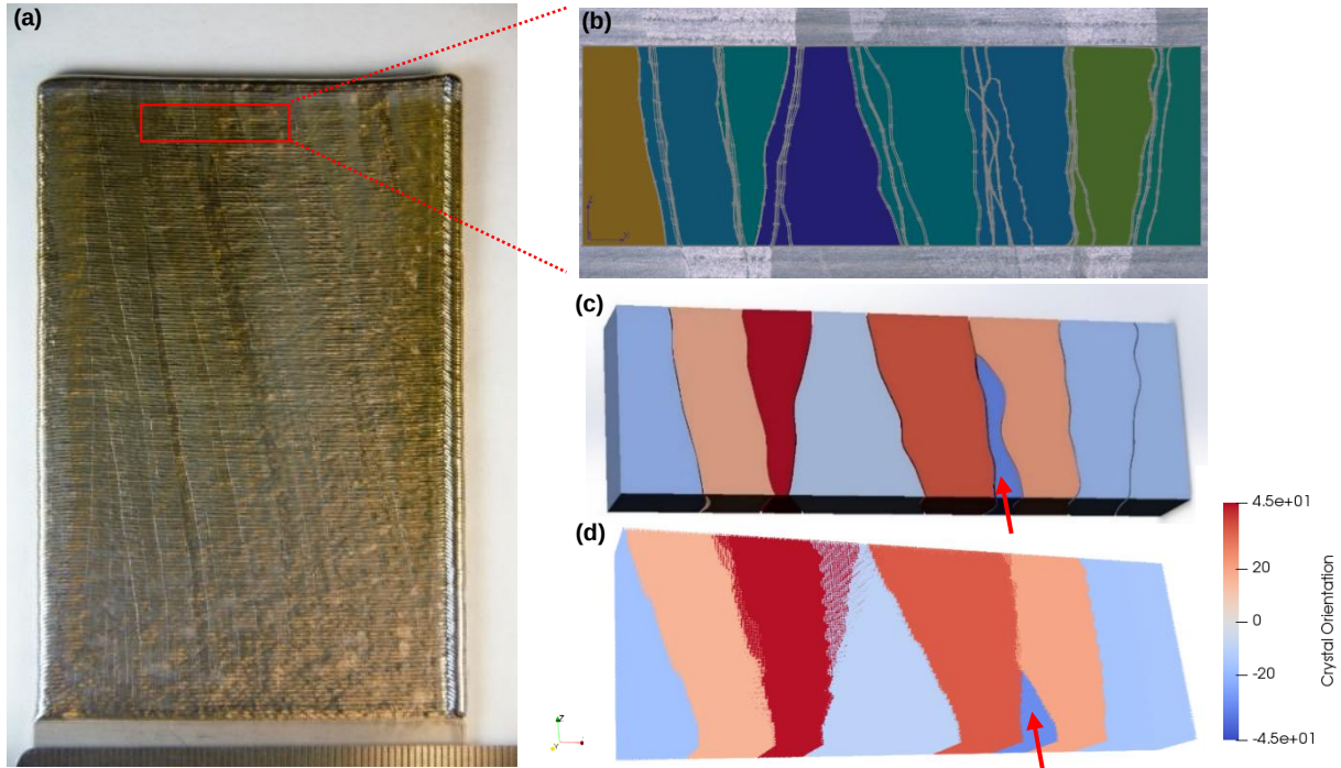
Figure 8: The application of the invasion model on the thin-wall structure. a. The simulation domain on a wire DED fabricated thin-wall structure. b. Grain boundary extraction on the three corresponding layers. c. Grain structure reconstruction result. d. Simulation result of the invasion model.
