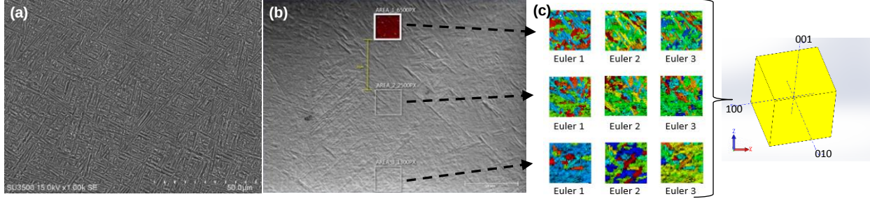
Figure 5: Microstructure of wire DED fabricated Ti6Al4V thin-wall structure. a. Electron microscope of the basketweave structure (fully \alpha' phase). b. Three detected areas (spaced at 50 \mu\text{m} ) within the same prior \beta grain. c. The three corresponding Euler angle maps of \alpha' grain and the reconstructed crystal orientation present of the prior \beta grain.
