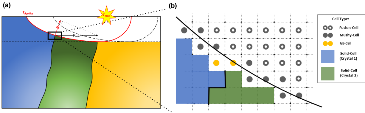
Figure 2: One timestep in the invasion model. a. Schematic of local solidification condition. b. Numerical representation of the simulation domain.
