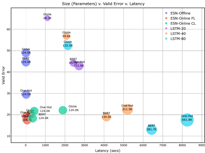
Fig. 12 GoLD (Large Data): Parameters vs Valid Error vs Latency.
