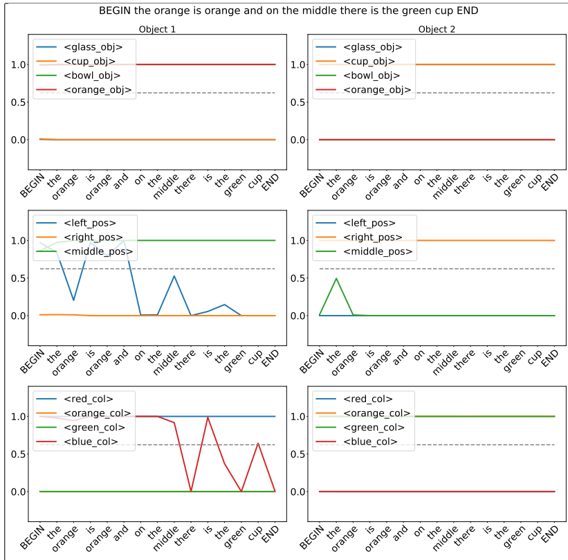
Fig. 14 Juven’s Data: Output activation of the ESN Offline + fine-tuned BERT. The activation are here shown after being transformed by the Sigmoid function.
