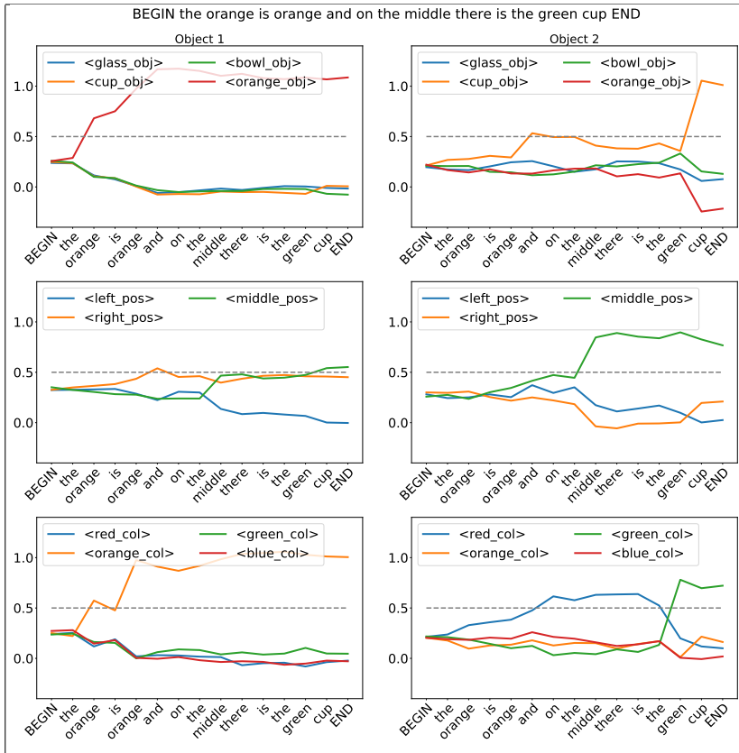
Fig. 16 Juven’s Data: Output activation of the ESN CL + fine-tuned BERT. After each word the model tries to predict the correct output. That’s why we can see a jump in the correct characteristic after the related keyword is seen.
