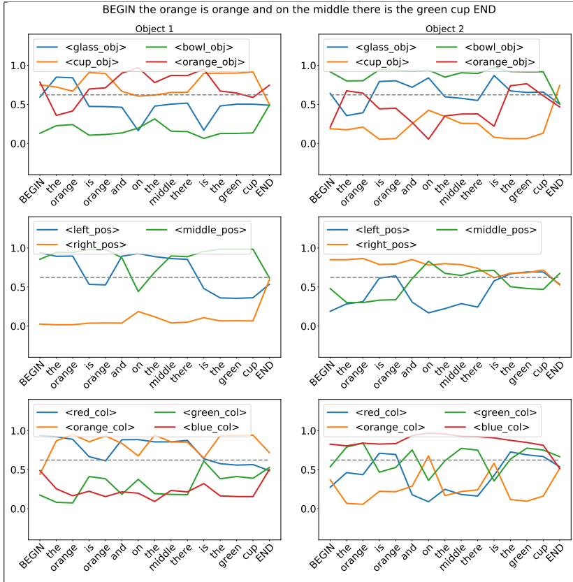
Fig. 15 Juven’s Data: Output activation of the ESN FL + fine-tuned BERT. The activation are here shown after being transformed by the Sigmoid function.
