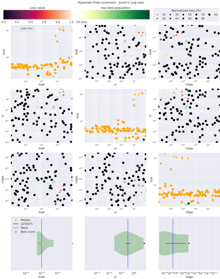
Fig. 8 Juven's data Cross-entropy loss: Hyper-parameter search dependence plot for CSL task.
