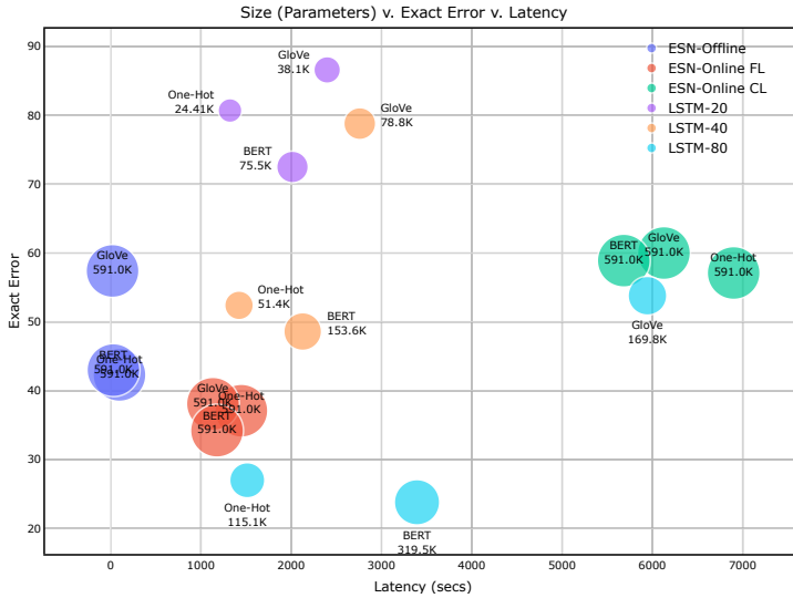
Fig. 13 Robot (Complex Corpora): Parameters vs Predicate Error vs Latency.
