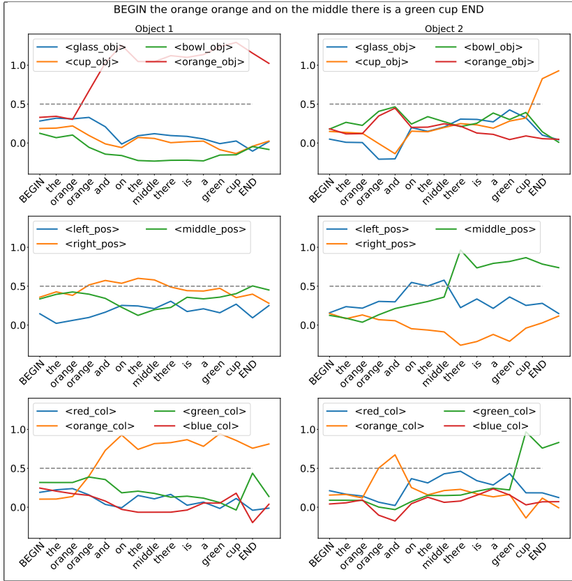
Fig. 17 Juven's Data: Output activation of the LSTM + fine-tuned BERT. Even if the learning procedure is only applied at the end, because of its learning algorithm, intermediate states are also optimized. This is why we can also interpret these transitional steps: they behave similarly to the ESN online trained with CL.
