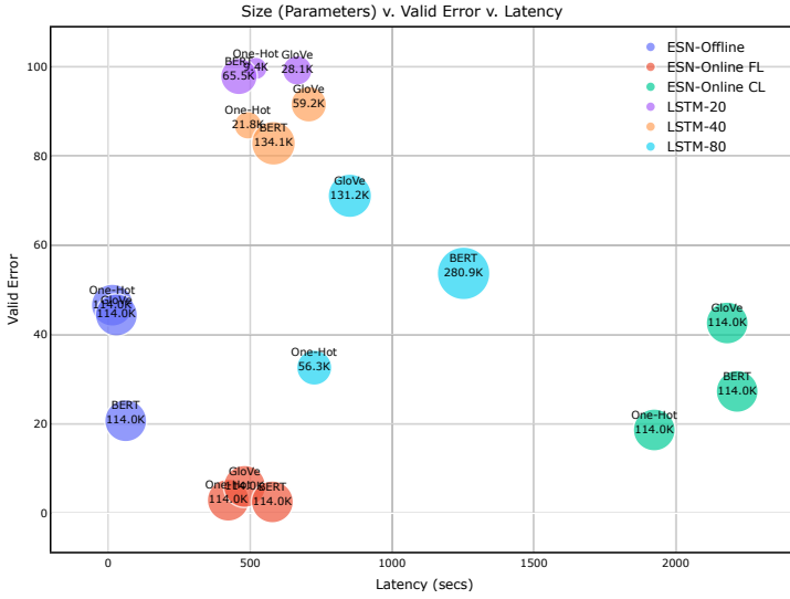
Fig. 11 Juven (Large Data): Parameters vs Valid Error vs Latency.
