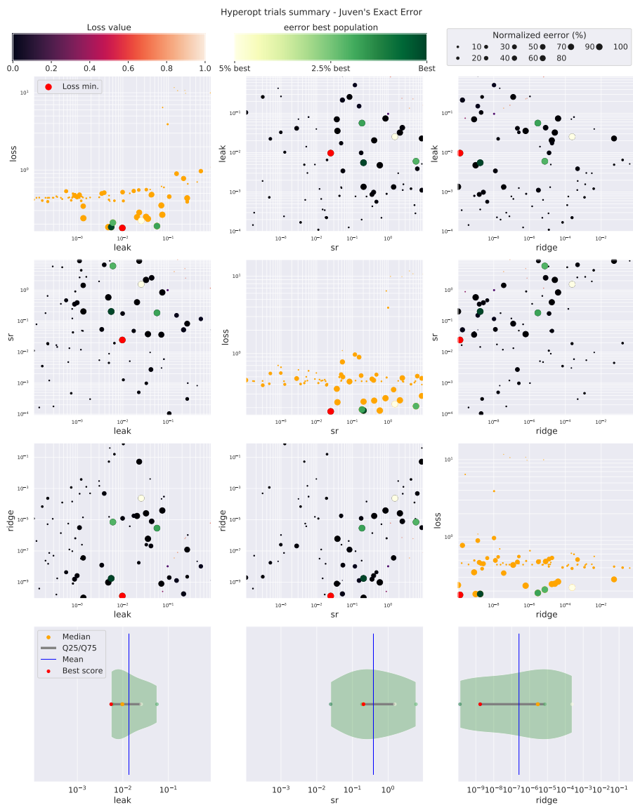
Fig. 10 Juven's data Exact Error: Hyper-parameter search dependence plot for CSL task.
