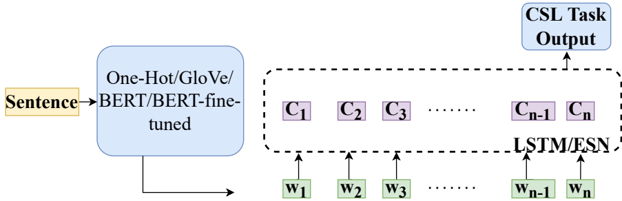
Fig. 2 Architecture of our CSL. The sentence are passed as input to One-Hot/GloVe/BERT/BERT-fine-tuned BERT for extracting the word embeddings. These token embeddings are passed as input to the LSTM/ESN models for the final prediction of CSL task outputs
