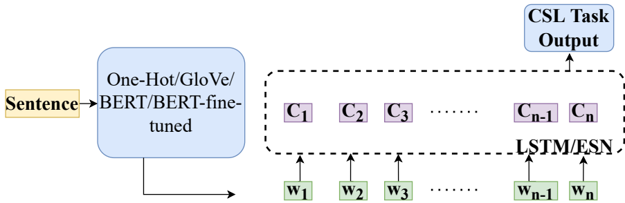
Fig. 2 Architecture of our CSL. The sentence are passed as input to One-Hot/GloVe/BERT/BERT-fine-tuned BERT for extracting the word embeddings. These token embeddings are passed as input to the LSTM/ESN models for the final prediction of CSL task outputs
