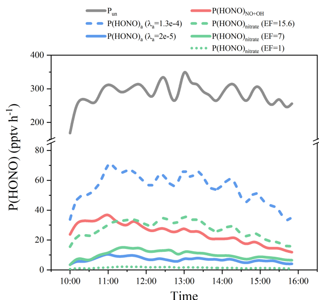
Figure 10. Unknown HONO source strength ( P_{\text{un}} ) and HONO production rates from \text{NO} + \text{OH} ( P(\text{HONO})_{\text{NO}+\text{OH}} ), \text{NO}_2 uptake on the aerosol surface ( P(\text{HONO})_{\text{a}} ) with the inferred \gamma_{\text{a\_inferred\_mini}} = 1.3 \times 10^{-4} and the popular used \gamma_{\text{a}} = 2 \times 10^{-5} , and nitrate photolysis ( P(\text{HONO})_{\text{nitrate}} ) with EF values of 1, 7, and 15.6.
