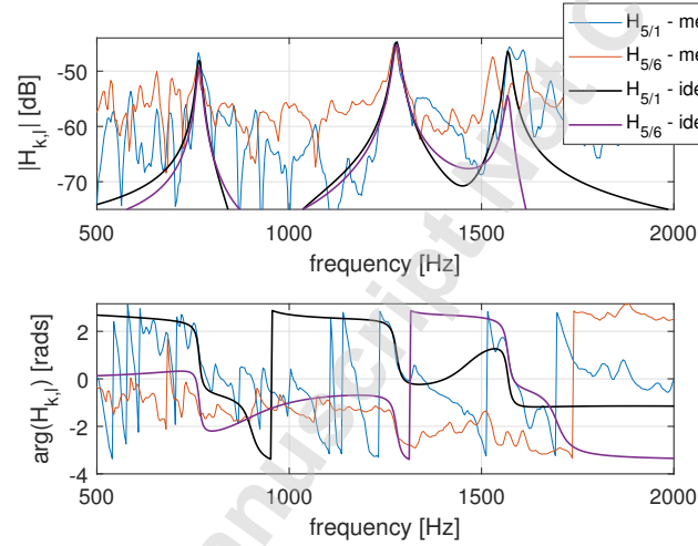
Fig. 11: Identification : FRF's of PZT n°5 to actuation (PZT 1 and 6), measurements and identifications from (1).
