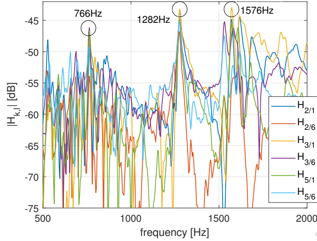
Fig. 8: FRF's of PZT sensors 2, 3, and 5 to actuation (PZT 1 and 6), targeted modes for control with zoom on the bandwidth of interest.
