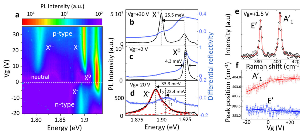
Fig. 2 Optical characterization of a charge tunable \text{MoS}_2 monolayer. a Photoluminescence (PL) intensity on a logarithmic scale under continuous wave (cw) laser excitation at 10 \mu\text{W} as a function of photon emission energy and gate bias V_g . b PL spectrum at a gate voltage corresponding to the p-type regime. c PL spectrum at a gate voltage corresponding to the neutral regime. d PL spectrum at a gate voltage corresponding to the n-type doping regime. Also shown is the differential reflectivity spectrum (filled dots) for each case. e Raman spectrum in the neutral regime, exhibiting the well-known E' and A'_1 vibrational modes. f Peak position for both modes of panel (e) as a function of gate bias. The error bars correspond to the uncertainty given by the fitting of the Raman spectrum with a double Lorentzian.
