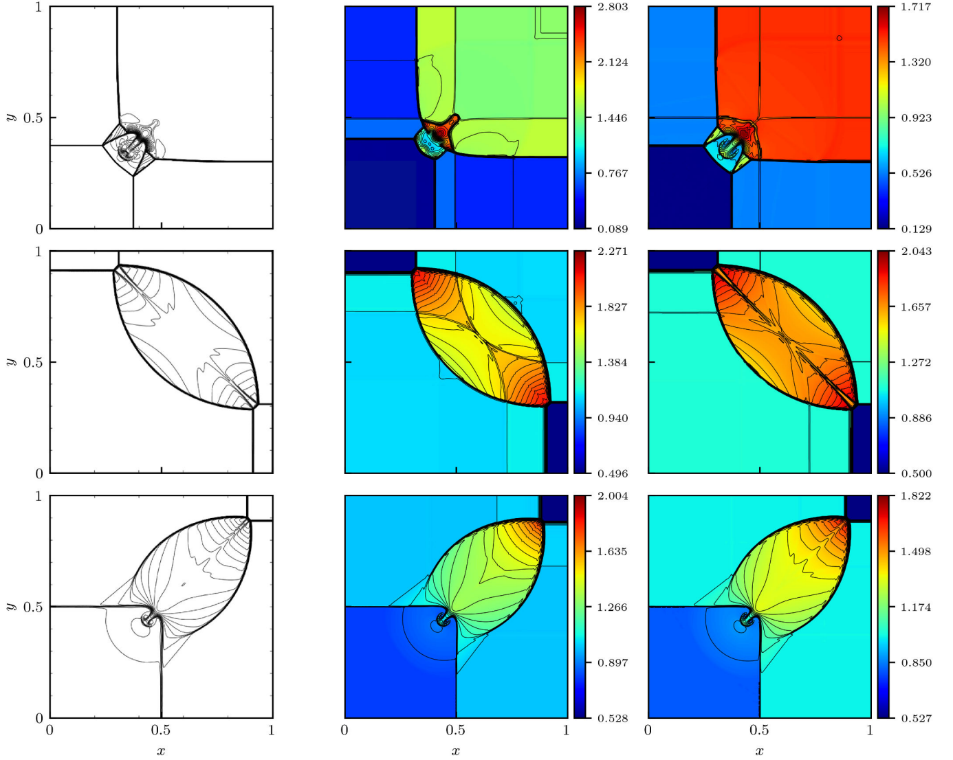
FIG. 11: Two-dimensional problems of Lax & Liu 75 . From left to right: reference 75 , s -MHM, \rho E -MHM. From top to bottom: density fields for configurations 3, 4 and 12 at time t = 0.3, 0.25 and 0.25 respectively.
