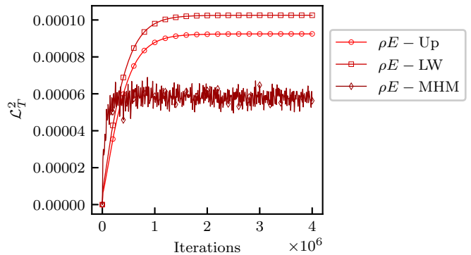
FIG. 1: Convergence study of the \mathcal{L}_T^2 error of the thermal Couette flow.
