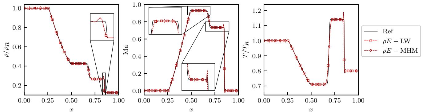
FIG. 10: Density, Mach and temperature profiles at time t = 0.2\sqrt{RT_L}/L in the Sod shock tube test case 71 , using the van Albada slope limiter for high-order LW and MHM schemes.
