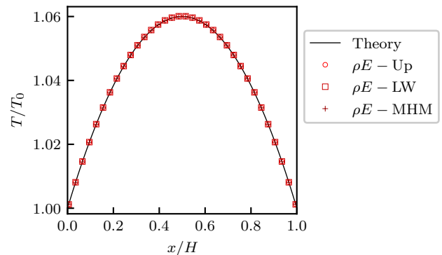
FIG. 2: Temperature profile of the thermal Couette flow.
