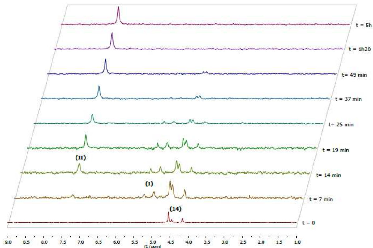
Fig. 2. 31 P NMR (101 MHz, acetone- d 6 ) following of prodrug 14 enzymatic hydrolysis by Carboxypeptidase Y.
