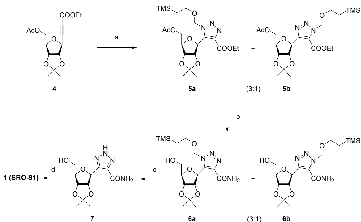
Scheme 2. Improved synthesis of 5-( \beta -D-ribofuranosyl)-2H-1,2,3-triazole-4-carboxamide (SRO-91): (a) \text{TMS}(\text{CH}_2)_2\text{OCH}_2\text{N}_3 , toluene, reflux (82%); (b) \text{NH}_3 gas, MeOH, rt (92%); (c) 1M TBAF in THF, reflux, then \text{CaCO}_3 , Amberlyst A21, rt, then \text{NH}_4\text{OH} , rt (51%); (d) DOWEX 50WX8, MeOH/ \text{H}_2\text{O} (4:1) 50°C (72%) or TFA, r.t. (86%)
