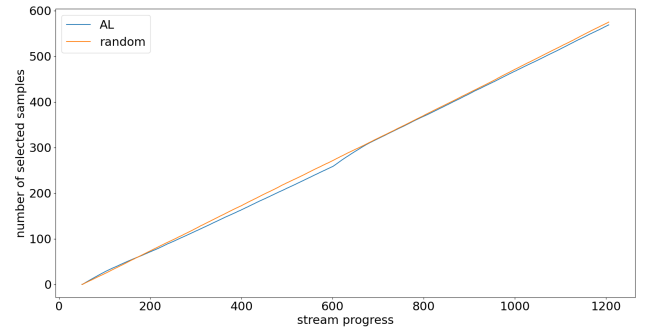
Fig. 4. Evolution of the average number of samples selected from the stream by either an AL or random strategies, over 100 runs of the experiment. The streams contain abrupt drift
