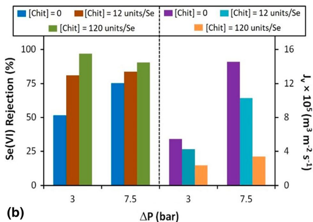
Fig. 9 Rejection and permeation flux obtained by ultrafiltration of solutions containing 1.7 mmol/L of a Se(IV) and b Se(VI) with and without chitosan at pH 4. CERAM 60 membrane, molecular weight cut off: 8 kDa
