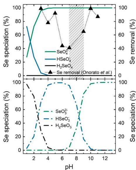
Fig. 7 Speciation of selenium VI (top) and IV (bottom), and removal of selenium VI, versus pH. Conditions: electric potential 12 V; feed salinity 5.3 g/L; membranes Neosepta CMX-SB & AMX-SB, Tokuyama Soda Ltd., Japan. The highlighted pH range shows the real pH of sample water used, which was then modified by adding HCl and NaOH. Adapted from Onorato et al. (2017)
