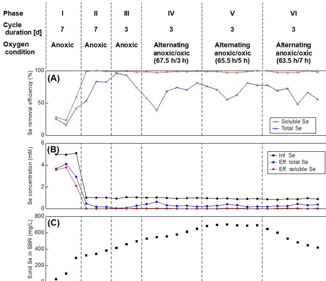
Fig. 11 Selenium removal performance of the sequencing batch reactor: A Se removal efficiencies, B Se concentrations in the influent and effluent, and C solid Se in the reactor. Adapted from Zhang et al. 2019
