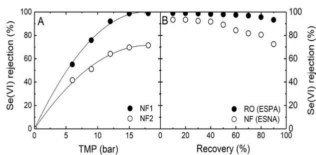
Fig. 6 Rejection of Se(VI) with nanofiltration/reverse osmosis membranes versus A transmembrane pressure (TMP) and B recovery. Sources: A) is adapted from Malhotra et al. (2020): Se(VI) 1600 µg/L and pH 8; B) is adapted from Chung et al. (2010): S(VI) 326 µg/L, pH 7.2 and pressure 8 bar
