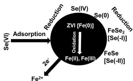
Fig. 4 Se(VI) adsorption and subsequent reduction to Se(IV), Se(0), Se(-I), and Se(-II) by zero-valent iron. This diagram shows the fractionation of selenium during the reduction of selenate by zero-valent iron, Se(VI) being reduced into various other species. The zero-valent iron technology involves complex redox and adsorption interactions between metallic iron and selenium oxyanions in the effluent, iron acting as a strong oxidant being the electron donor and as a catalyst for oxyanion reduction. Adapted from Shrimpton et al. (2015)
