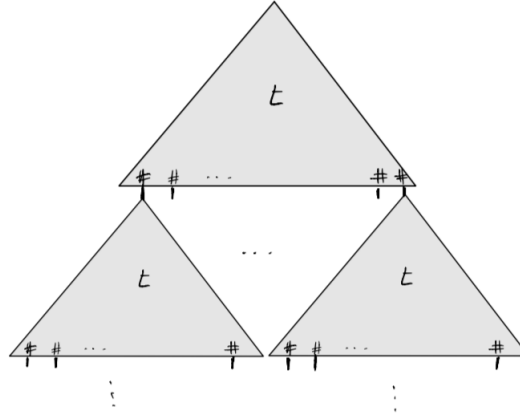
■ Figure 8 Strategy \sigma_t constructed from a \Sigma -tree t .
