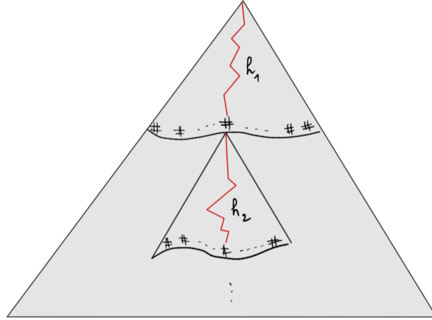
1020 Figure 9 Losing play \pi = \#h_1\#h_2\#\dots constructed from a strategy \sigma , seen as a tree.
